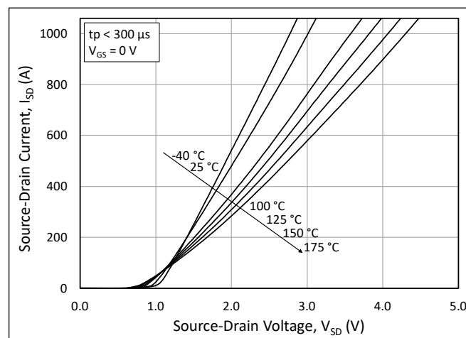
Figure 6. 3 rd Quadrant Characteristic vs. Junction Temperatures at V_{GS} = 0\text{ V} (Diode)
