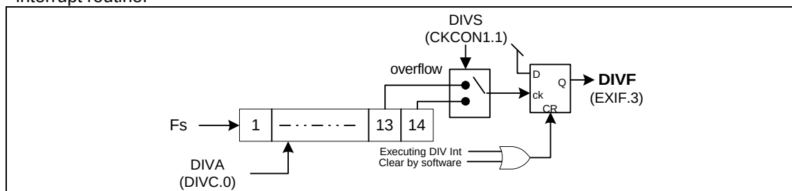
Figure 6-13 13/14-bit Divider
