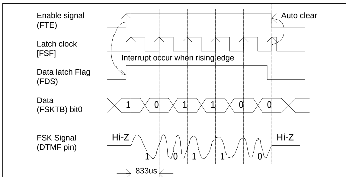
Figure 6-12 FSK Modulator
