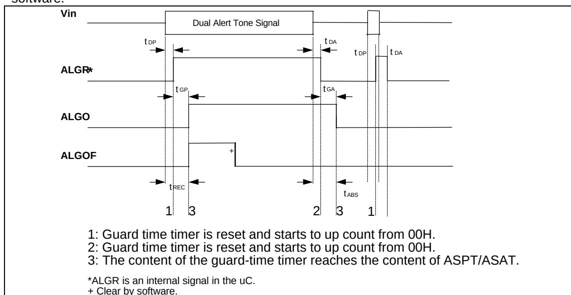
Figure 6-21 Guard Time Waveform of Alert Tone Signal Detection
