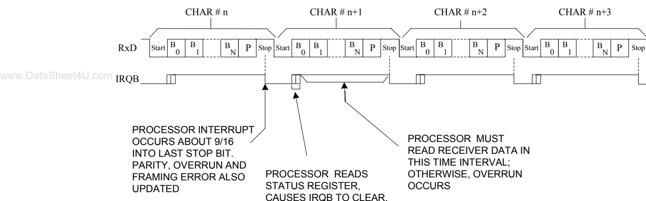
Figure 7 Continuous Data Receive
