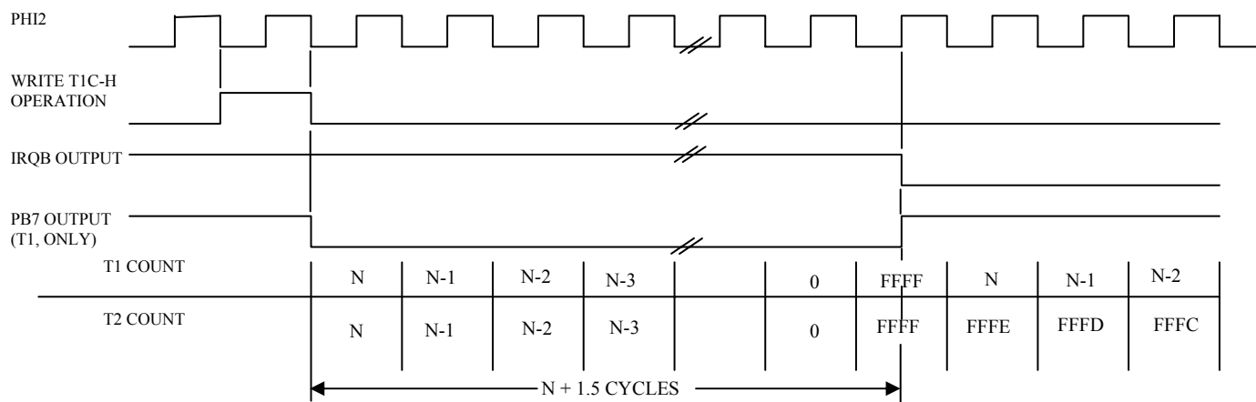
Figure 1-3 One-Shot Mode (Timer 1 and Timer 2)
