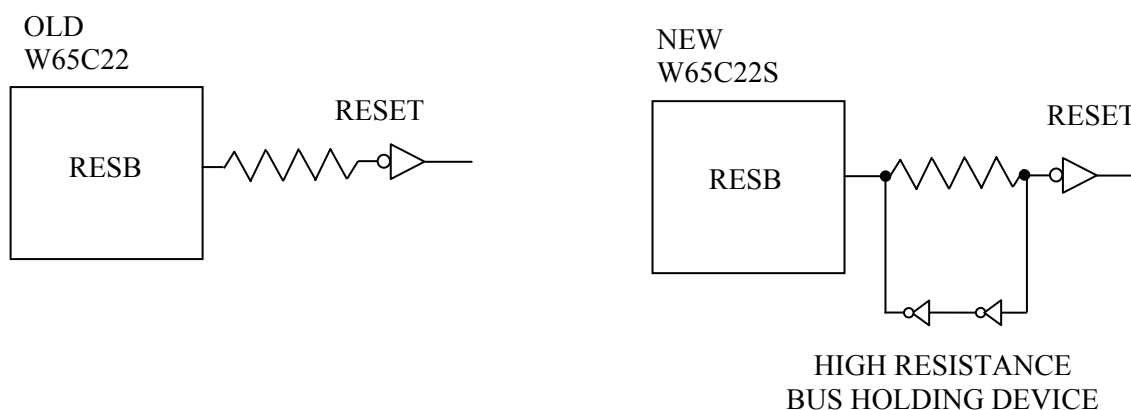
Figure 4-2 High Resistance Bus Holding Device
