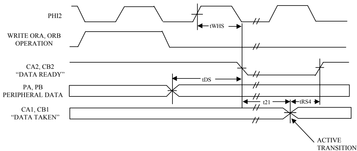
Figure 3-7 Write Handshake, Handshake Mode Timing (CA2, CB2)
