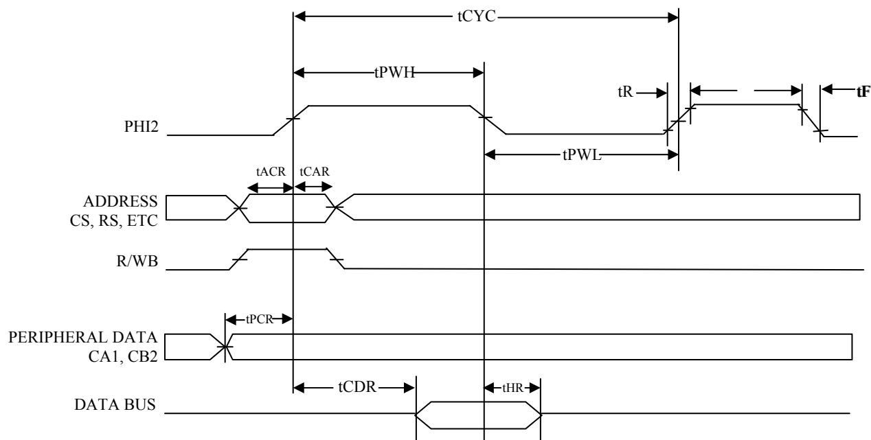
Figure 3-2 Read Timing
