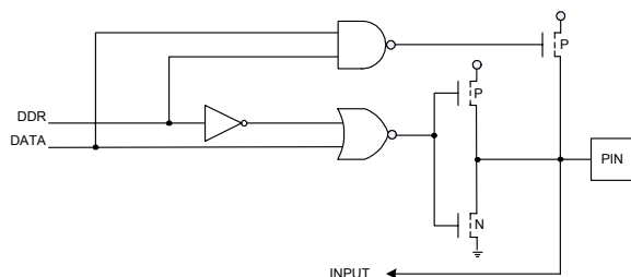
Figure 9 Port A, CA2 Buffers
