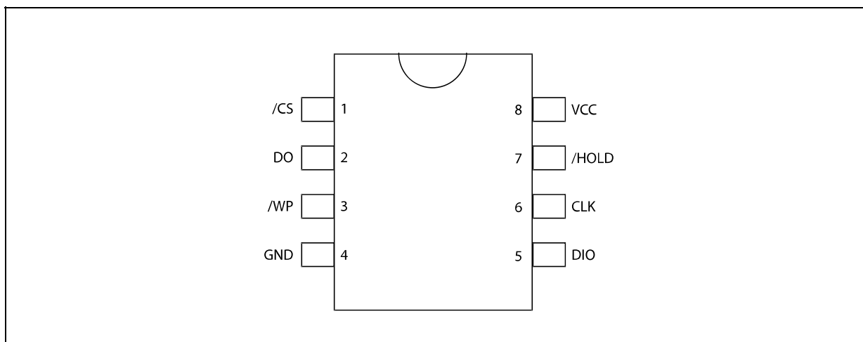
Figure 1c. W25X40A and W25X80A Pin Assignments, 8-pin PDIP (Package Code DA)
