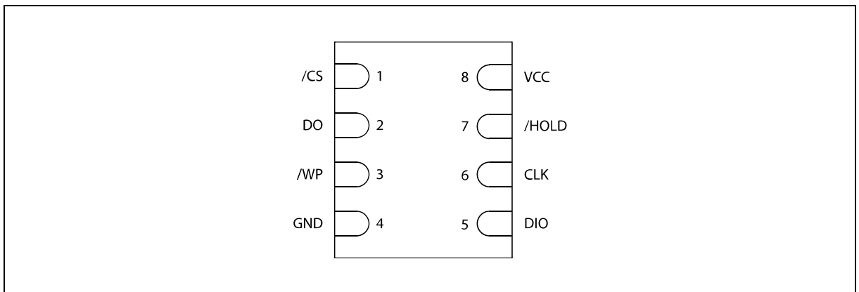
Figure 1b. W25X32BV Pad Assignments, 8-pad WSON 6x5-mm (Package Code ZP) and 8x6-mm (Package Code ZE)
