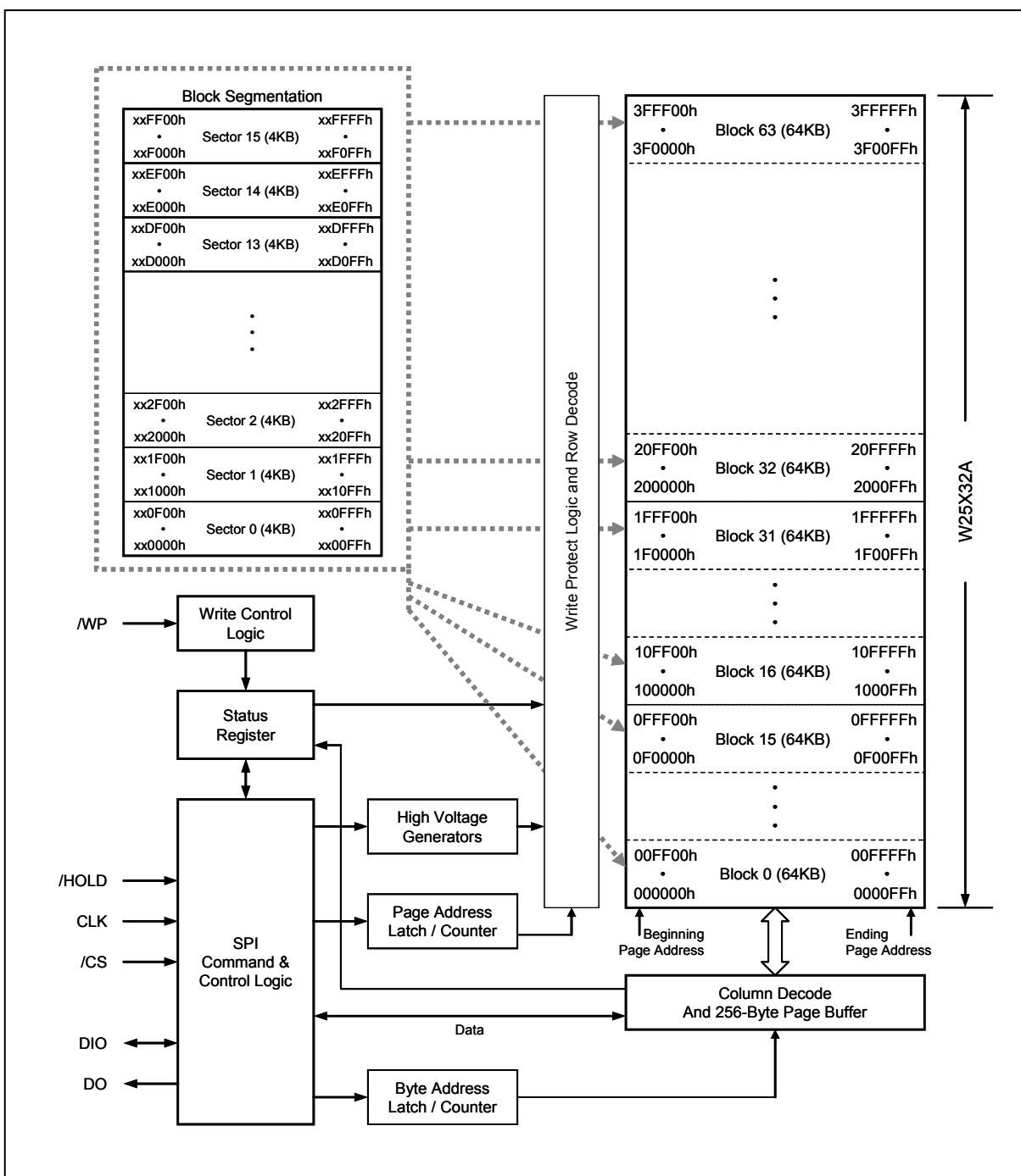
Figure 2. W25X32A Serial Flash Memory Block Diagram
