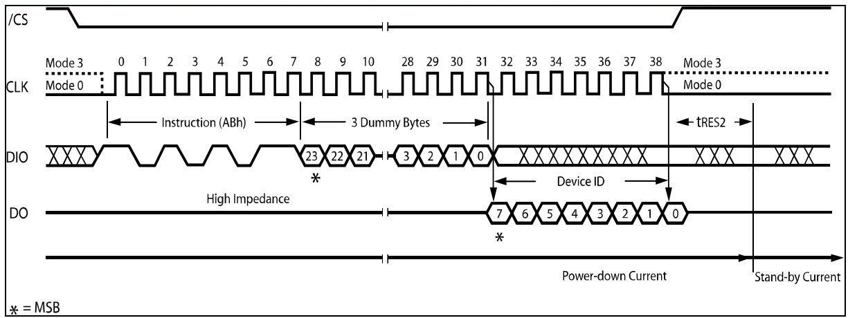
Figure 21. Release Power-down / Device ID Instruction Sequence Diagram
