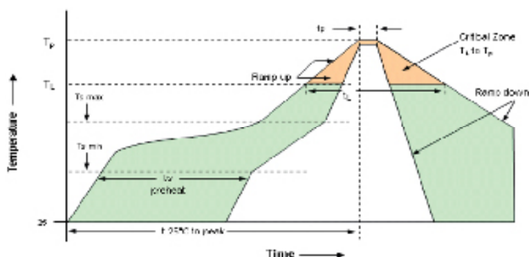
Solderprofile:
