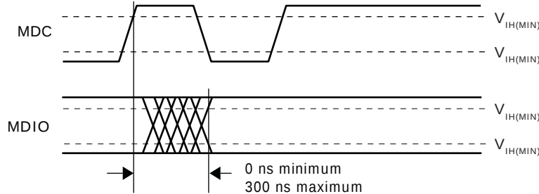
Figure 50 • Timing with MDIO Sourced by MMD
