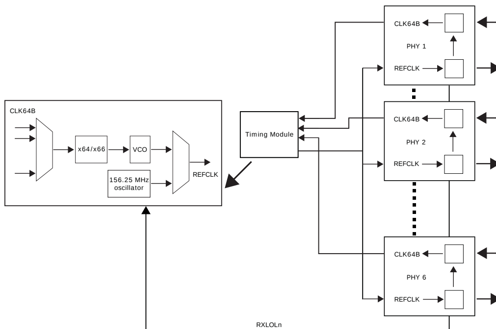
Figure 58 • Clock Path Distribution, Conventional Mode
