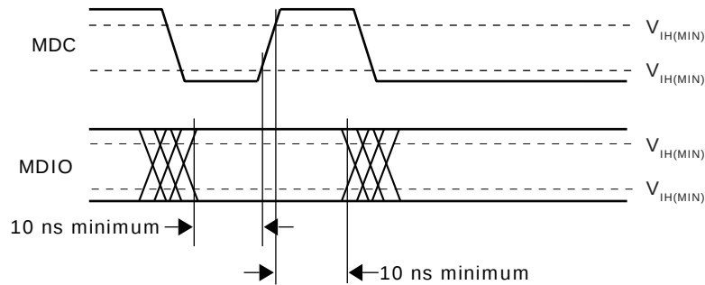
Figure 70 • Timing with MDIO Sourced by MMD
