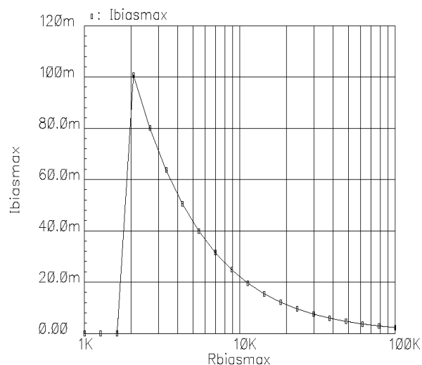
I_{BIASMAX} vs. R_{BIASMAX} T=25^{\circ}\text{C} , V_{CC} = 3.3\text{V}
