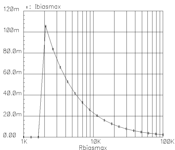
I_{BIASMAX} vs. R_{BIASMAX} T=25^{\circ}\text{C} , V_{CC} = 5\text{V}
