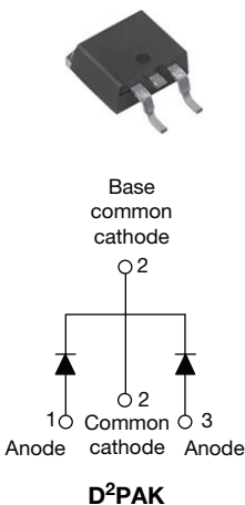
VS-10CTQ150SPbF
