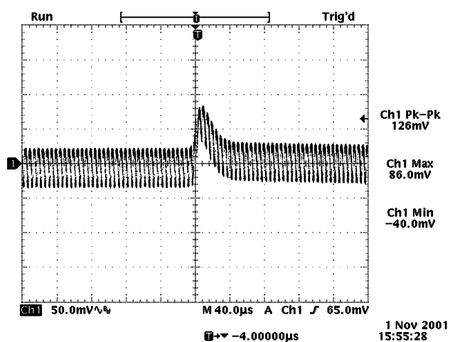
100% to 50% load transients at 12V input and T_a=25^\circ\text{C}
