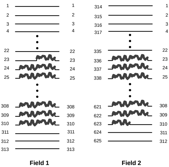
Fig. 2–35: Mapping for 625/50 line systems
