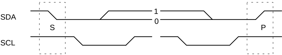
Fig. 2–41: I 2 C bus protocol (MSB first)
