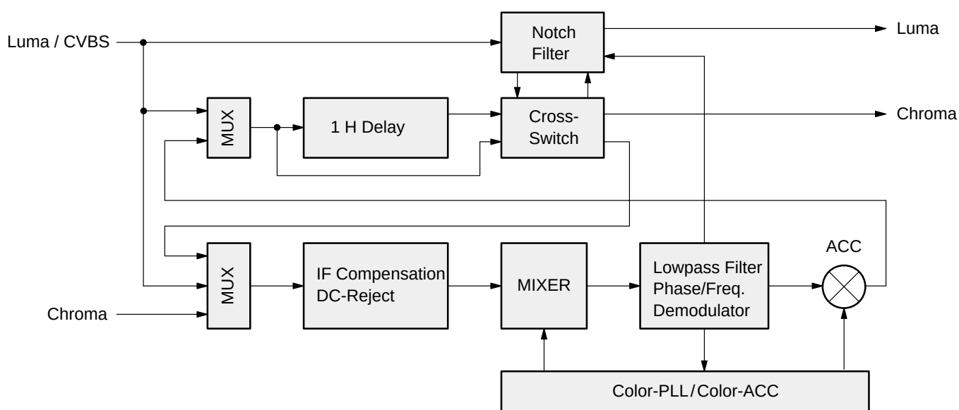
Fig. 2–5: Color decoder
