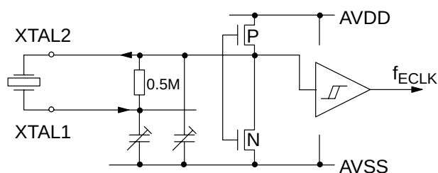
Fig. 3-10: Crystal Oscillator
