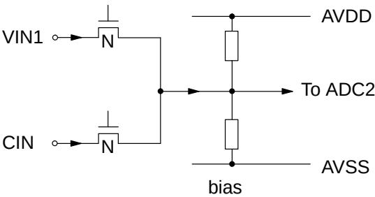
Fig. 3–13: Video Inputs ADC2
