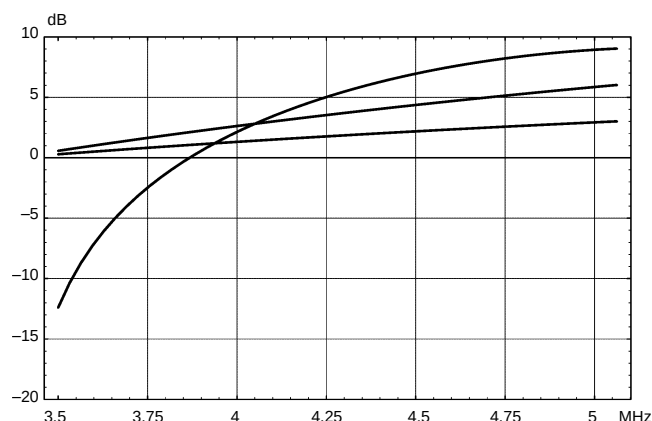
Fig. 2–4: Freq. response of chroma IF-compensation
