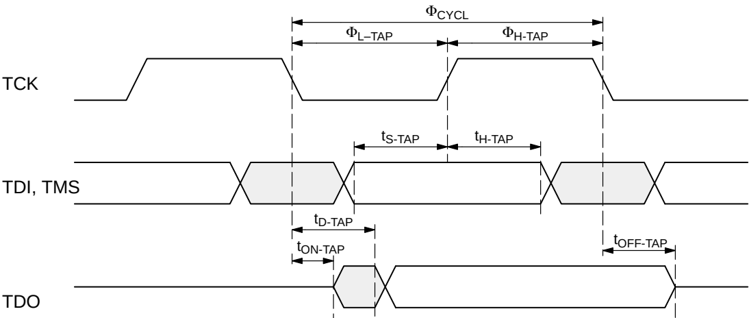
Fig. 5–5: Timing of Test Access Port TAP
