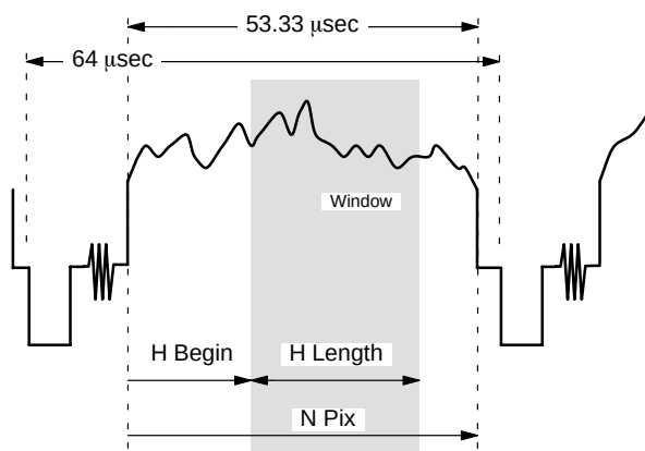
Fig. 2–33: Horizontal dimensions of sampling window
