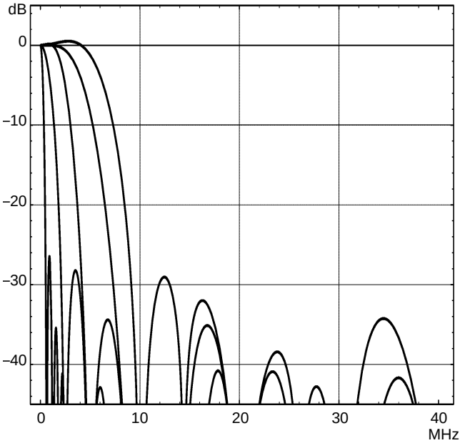
Fig. 2–13: Freq. response of 5 widely spaced filters
