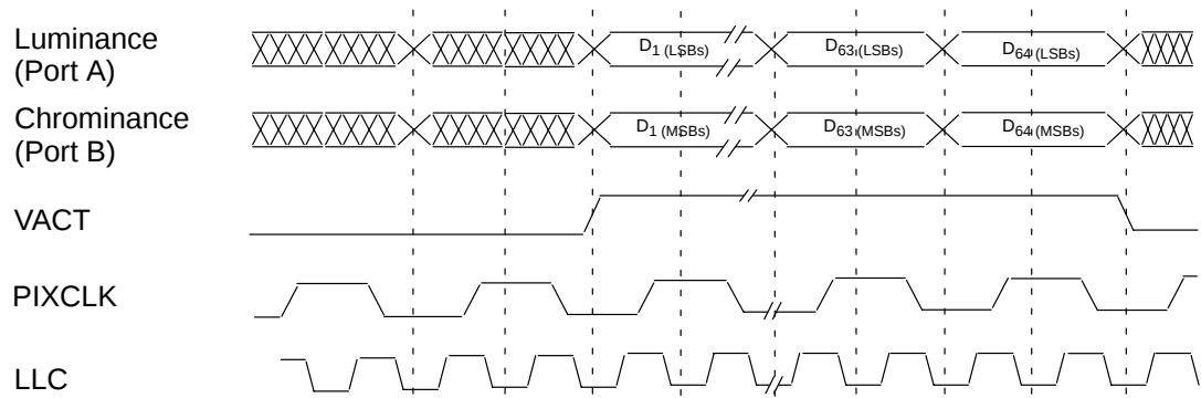
Fig. 2–42: Timing during lines with sliced VBI-data (single clock)
