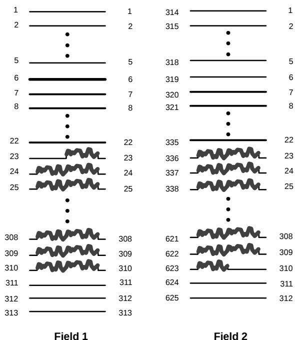
Fig. 2-38: Mapping for 625/50 line systems
