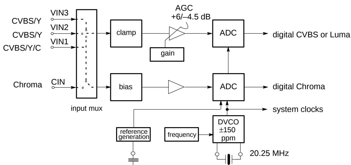
Fig. 2–1: Analog front-end
