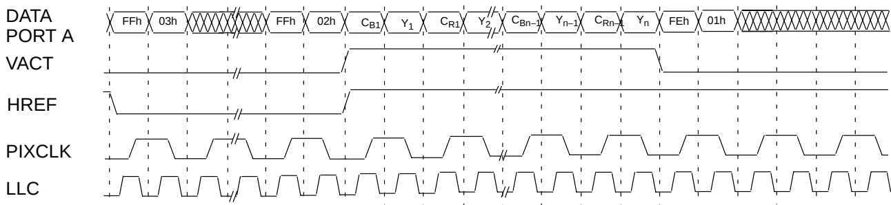
Fig. 2–27: Output of video or VBI-data with timing event codes (BStream); double clock on
