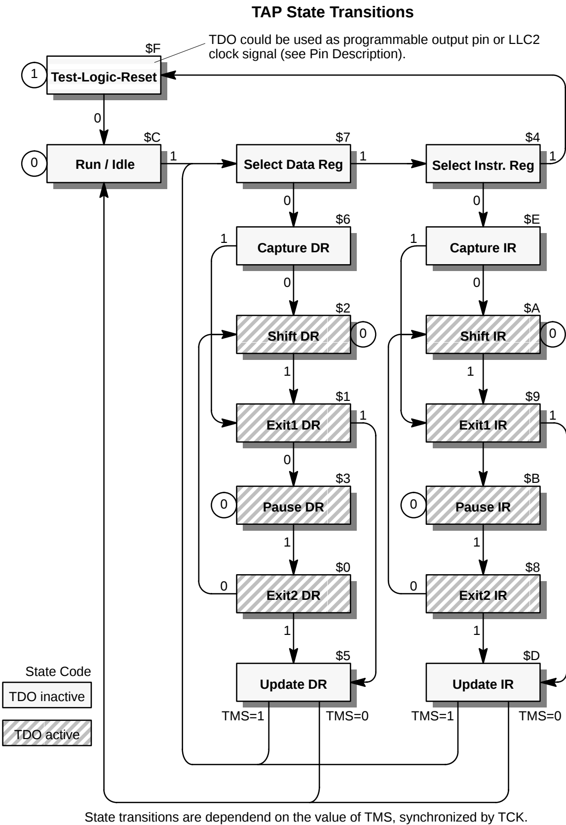
Fig. 2-48: TAP state transitions
