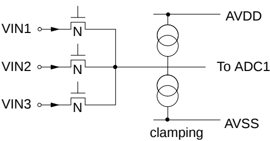
Fig. 3-10: Video Inputs ADC1
