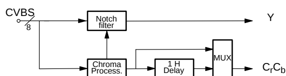
Fig. 2–9: SECAM color decoding
