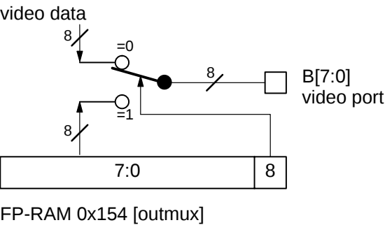
Fig. 2–26: Programmable output port
