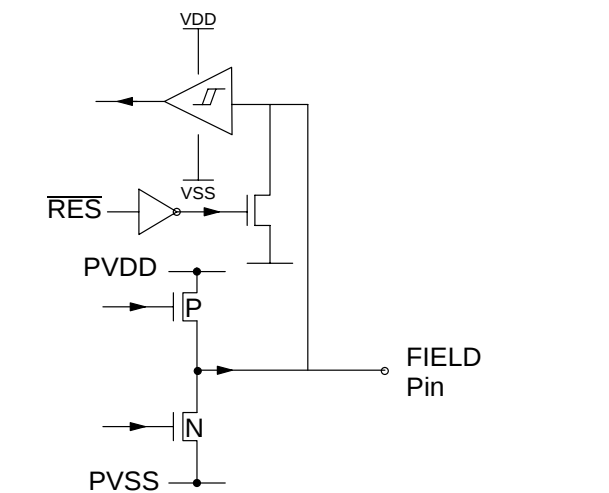
Fig. 3-7: Reference Signal FIELD and wake-up selection LOWPOW on positive edge of \overline{\text{RES}}
