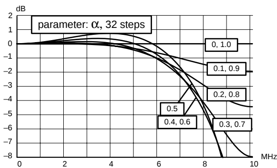
Fig. 2–16: Luminance skew filter magnitude frequency response
