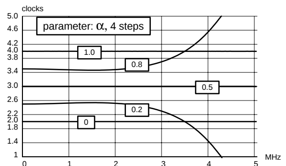
Fig. 2–19: Chrominance skew filter group delay characteristics
