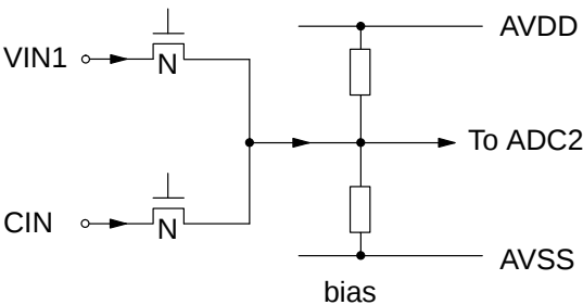
Fig. 3-11: Video Inputs ADC2
