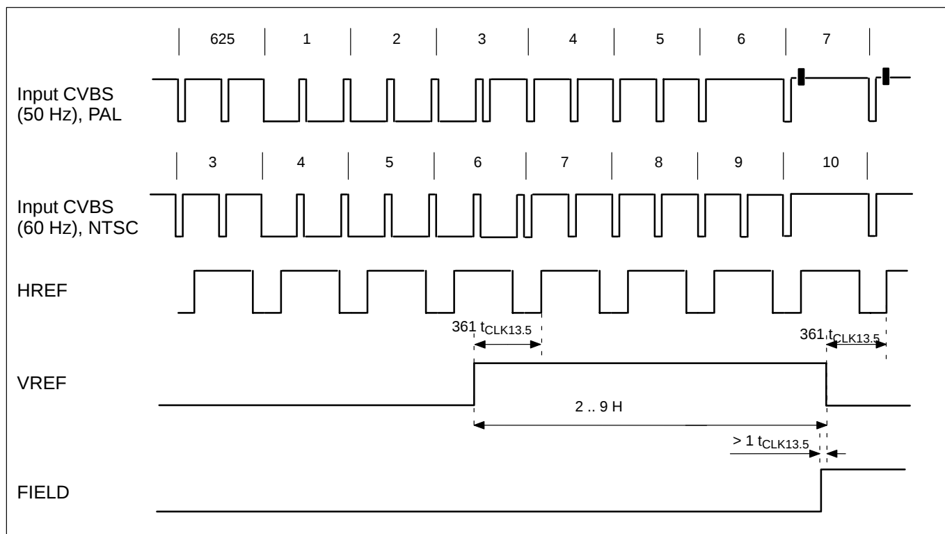
Fig. 2-33: VREF timing for ODD fields
