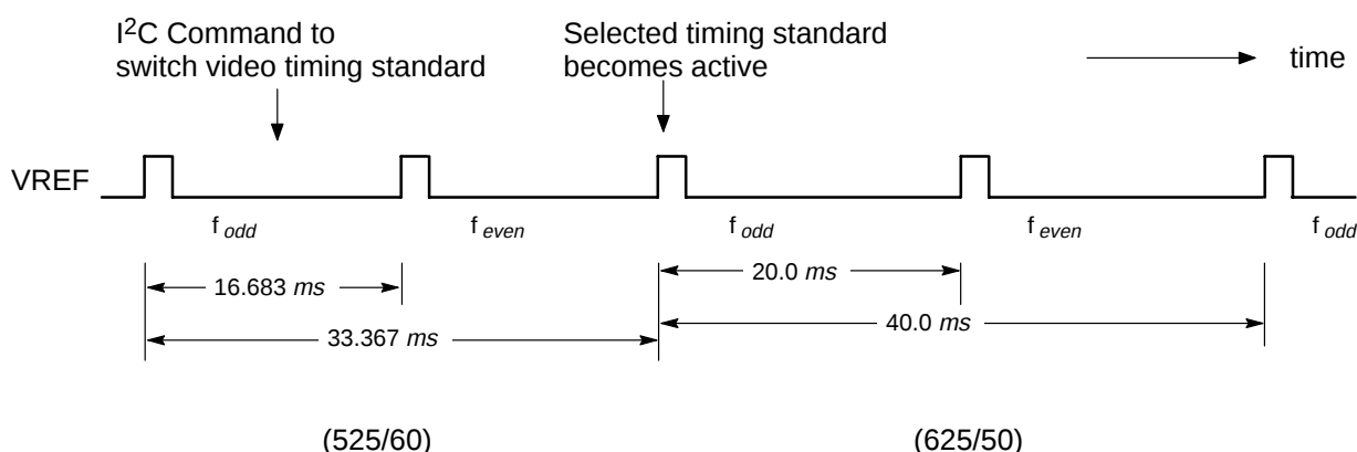
Fig. 2–43: Transition between timing standards
