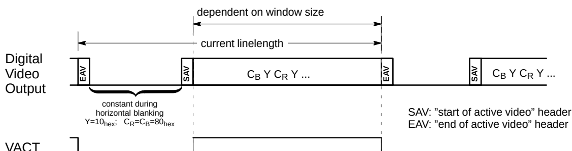
Fig. 2–23: Output of video or VBI data with embedded reference headers (according to ITU-R656)
