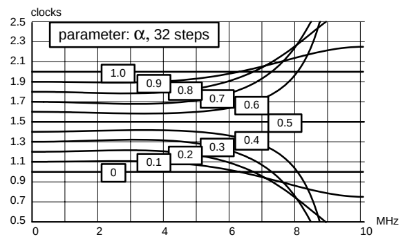
Fig. 2–17: Luminance skew filter group delay characteristics
