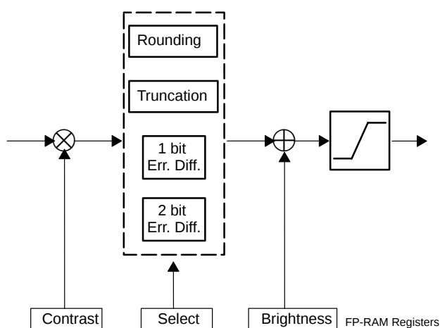
Fig. 2–20: Contrast and brightness adjustment
