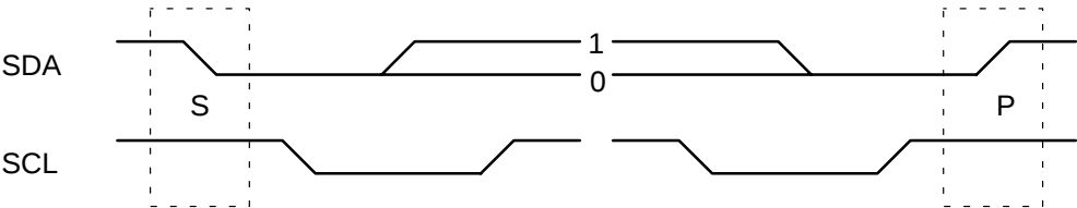
Fig. 2–46: I 2 C bus protocol (MSB first)
