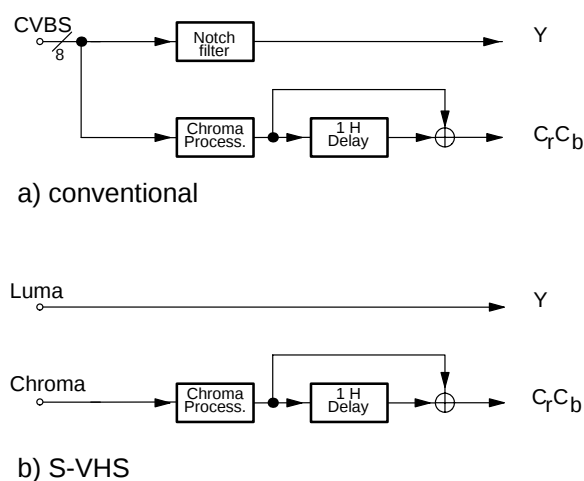
Fig. 2–7: PAL color decoding options
