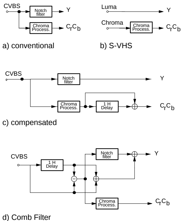
Fig. 2–6: NTSC color decoding options
