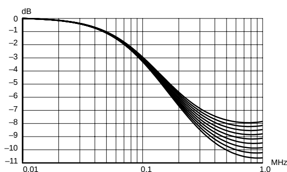
Fig. 2-5: Frequency response of SECAM deemphasis
