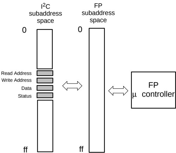
Fig. 4–2: FP register addressing
