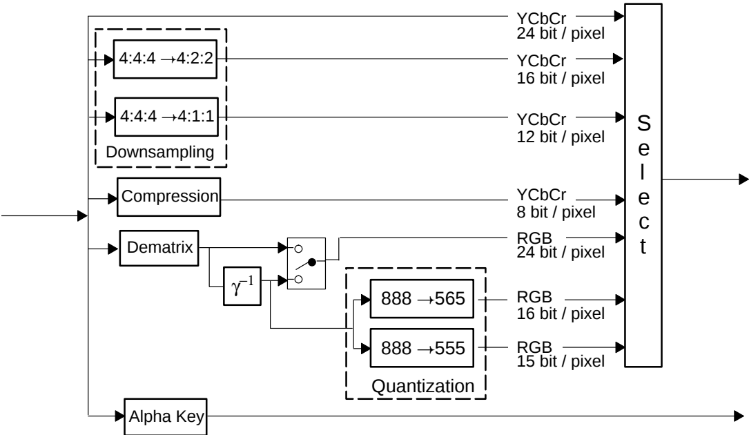
Fig. 2–19: The color space stage
