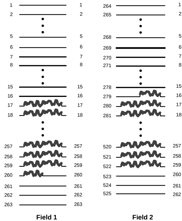
Fig. 3–7: Mapping for 525/60 line systems
