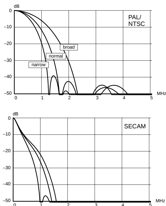
Fig. 2-4: Frequency response of chroma filters
