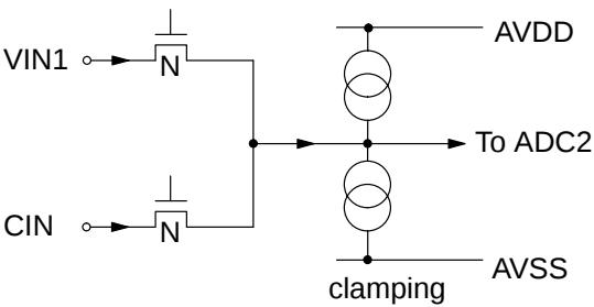
Fig. 6-14: Video Inputs ADC2
