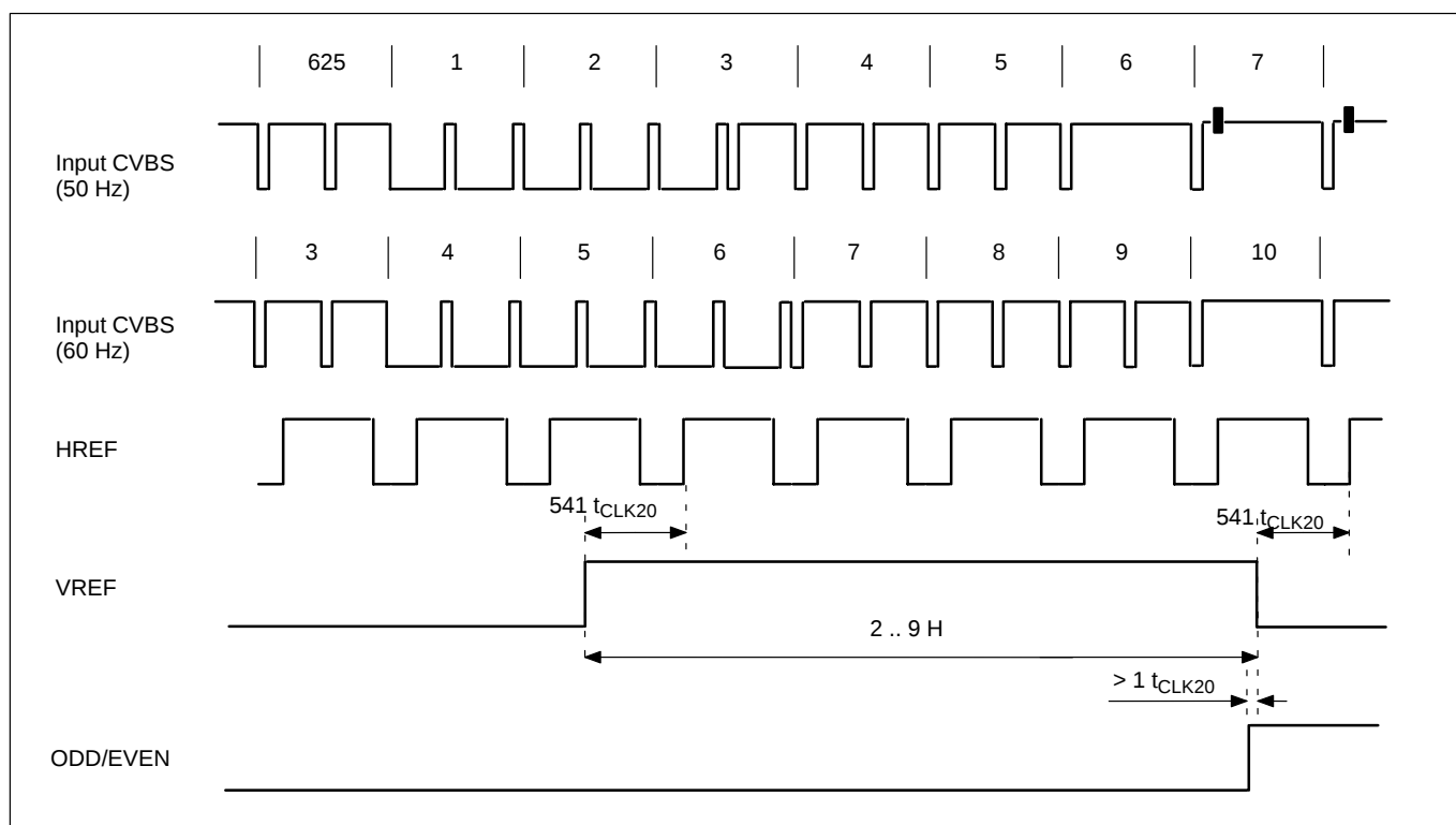
Fig. 3-2: VREF timing for ODD fields
