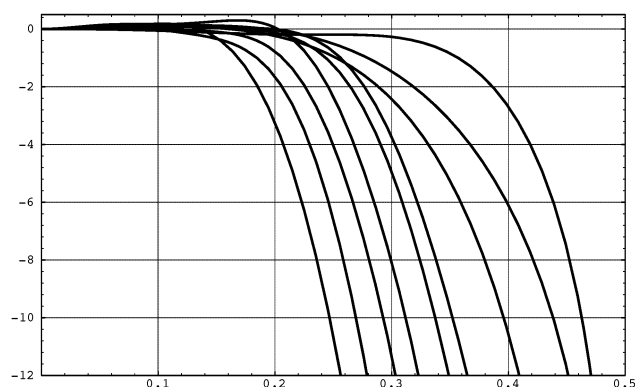
Fig. 2–11: Resizer filters for the upper octave
