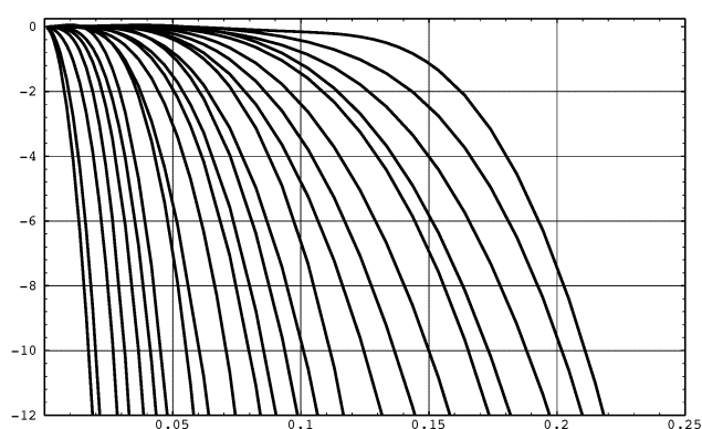
Fig. 2–12: Resizer filters for the lower three octaves
