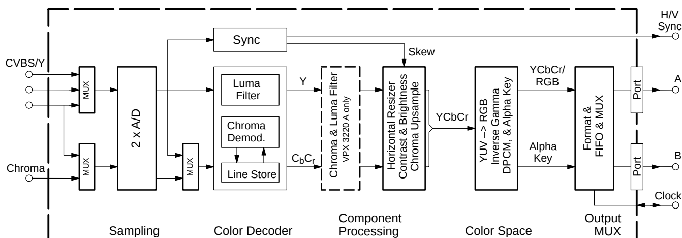
Fig. 1–1: Block diagram of the VPX
