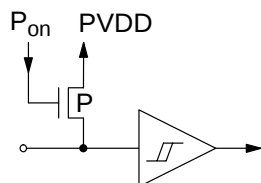
Fig. 6-6: JTAG Inputs TMS, TDI
