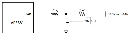
Figure 4. Shutdown Operation
