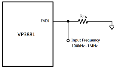
Figure 3. Clock Synchronization
