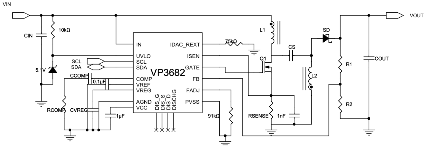
Figure 12. VP3682 Typical SEPIC Application
