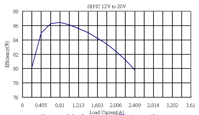
Figure 20. Example Efficiency(3)
