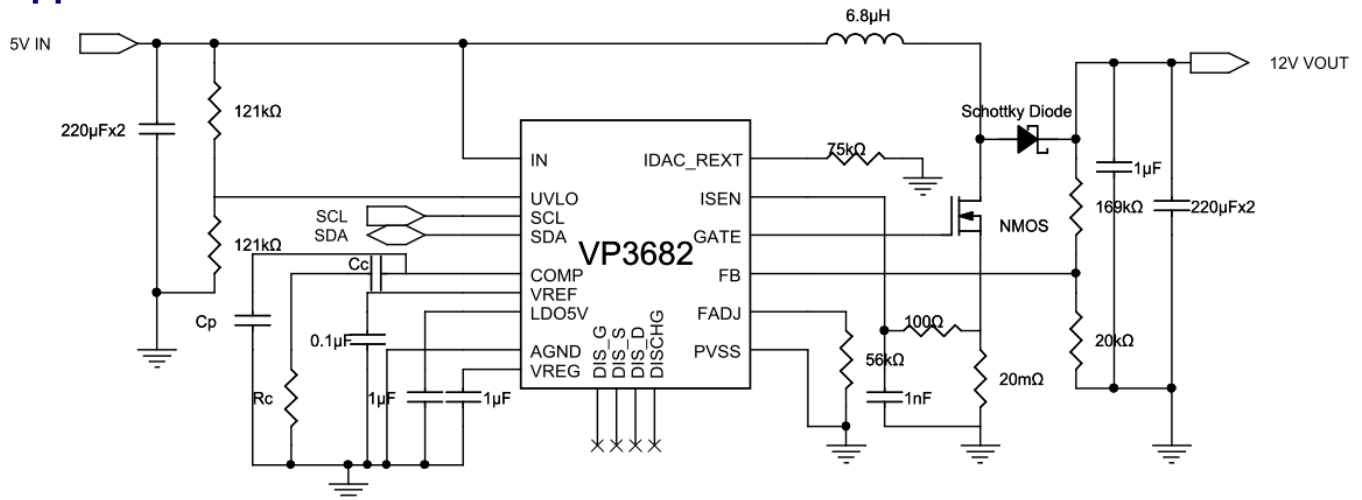
Figure 7. VP3682 Typical Boost Application
