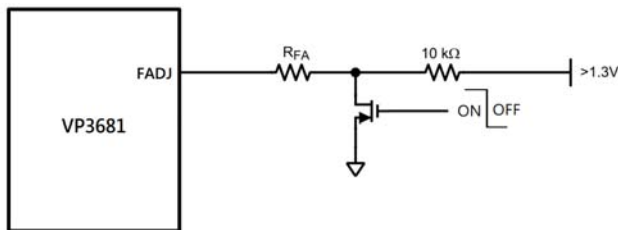
Figure 4. Shutdown Operation
