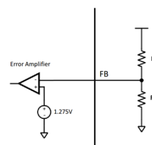
Figure 5. FB Pin Resistor Network
