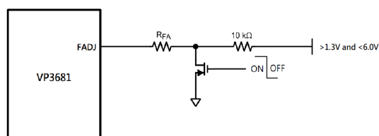
Figure 4. Shutdown Operation
