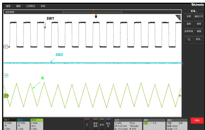
Figure 14. Forced CCM Operation (Buck)
