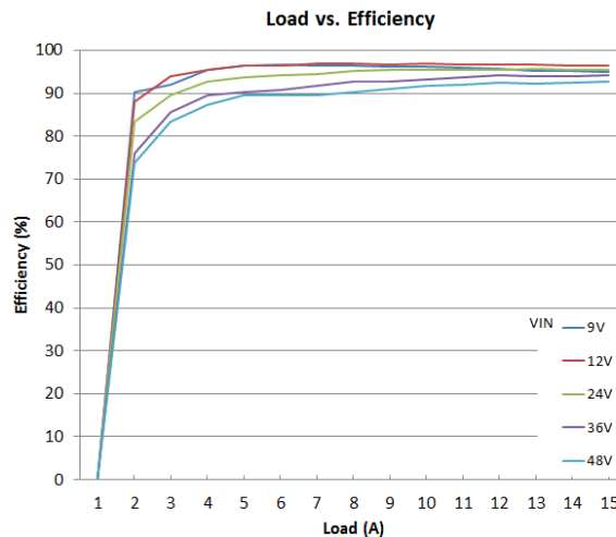
Figure 9. Efficiency ( V_{IN} )
