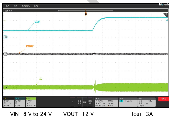
Figure 12. Line Transient
