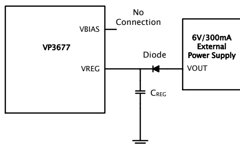
Figure 5. External VREG Supply
