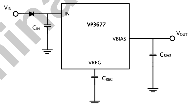
Figure 3. VREG and VBIAS
