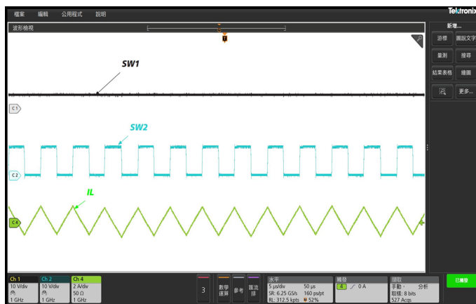
Figure 15. Forced CCM Operation (Boost)
