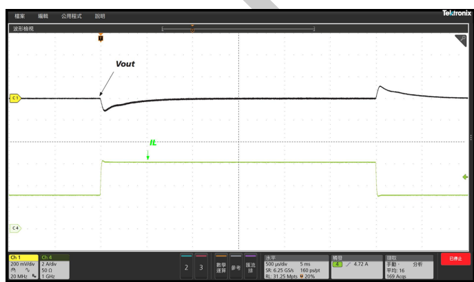
Figure 18. Load Step (Boost)
