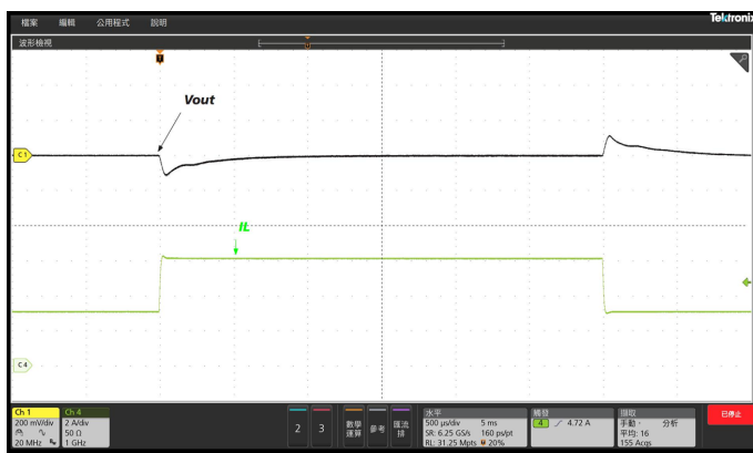
Figure 19. Load Step (Buck-Boost)
