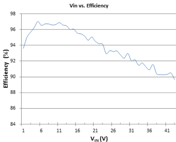
Figure 8. Efficiency ( I_{OUT}=2A )
