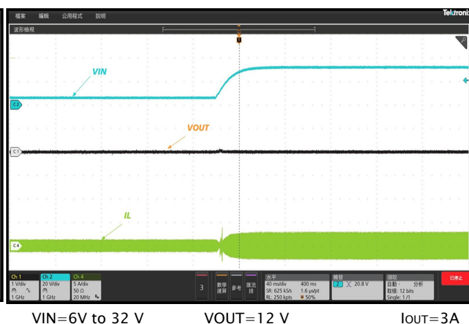
Figure 13. Line Transient
