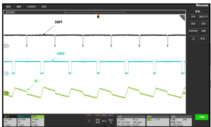
Figure 16. Forced CCM Operation (Buck-Boost)
