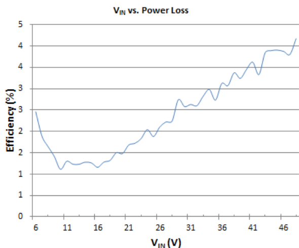
Figure 10. Power Loss ( I_{OUT}=2A )
