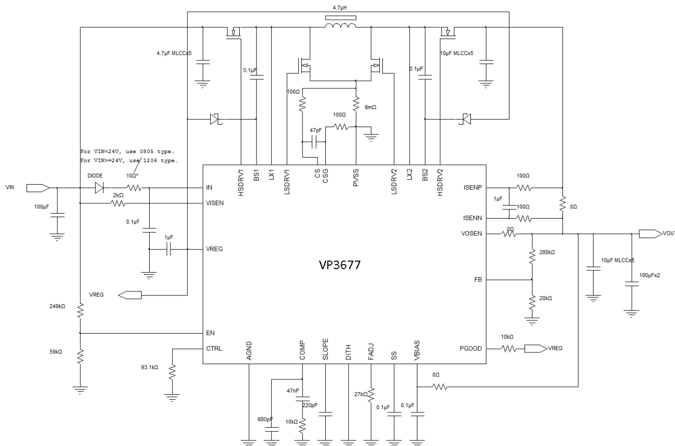
Figure 7. VP3677 Typical Application
