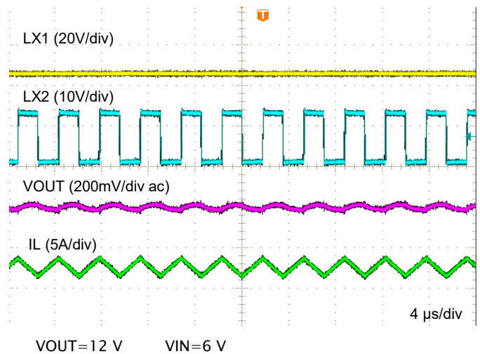
Figure 17. Forced CCM Operation (Boost)
