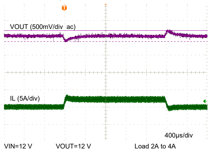
Figure 21. Load Step (Buck-Boost)
