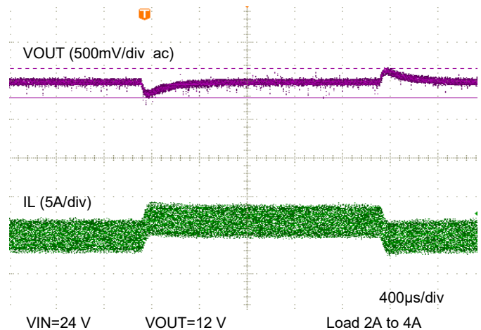
Figure 19. Load Step (Buck)
