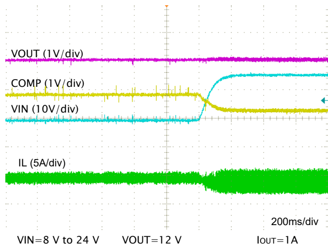
Figure 23. Line Transient
