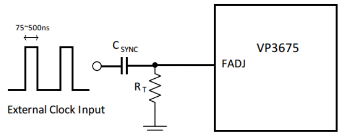
Figure 2. External Clock Synchronization
