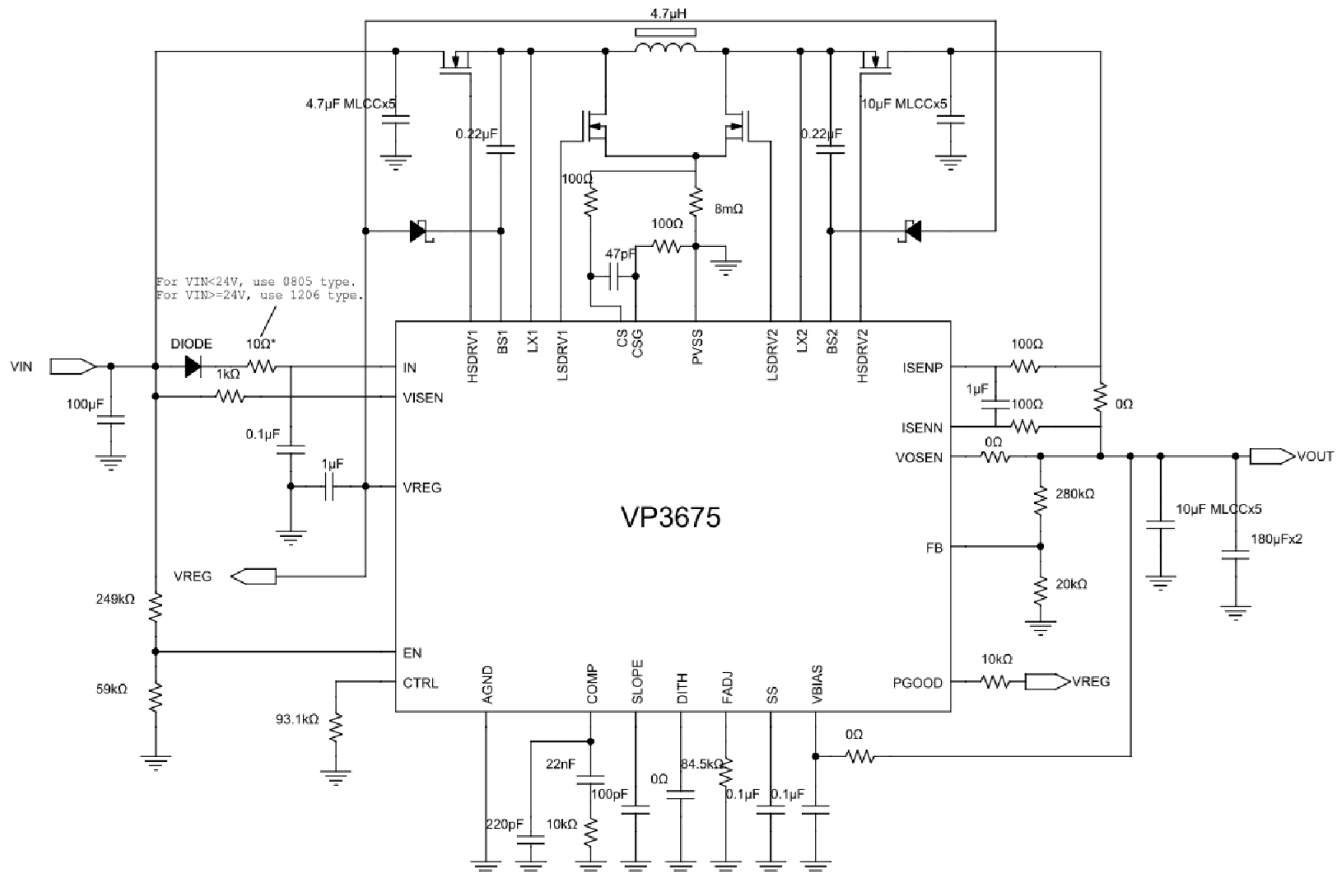
Figure 5. VP3675 Typical Application
