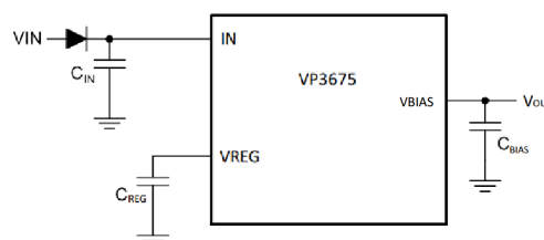
Figure 3. VREG and VBIAS
