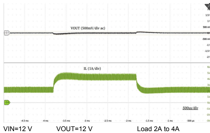
Figure 18. Load Step (Buck-Boost)
