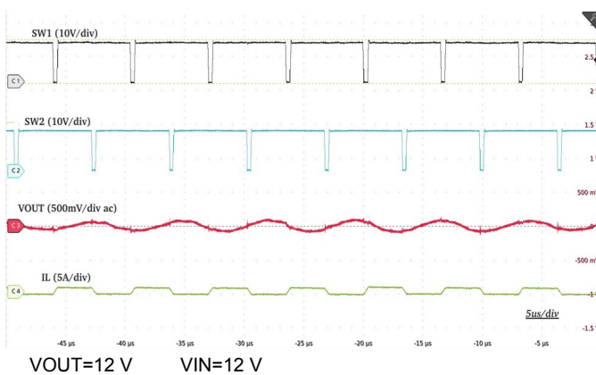
Figure 14. Forced CCM Operation (Buck-Boost)
