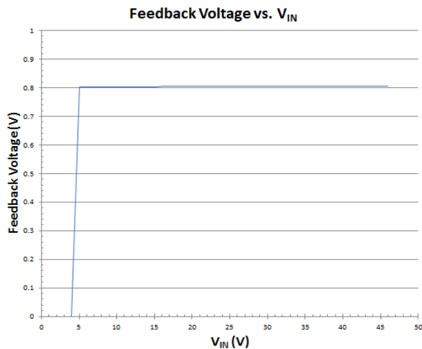
Figure 12. V_{FB} vs. V_{IN}
