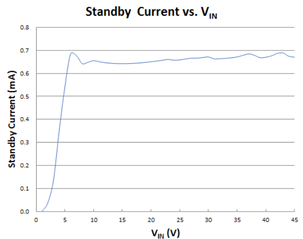
Figure 10. Standby Current vs. V_{IN}
