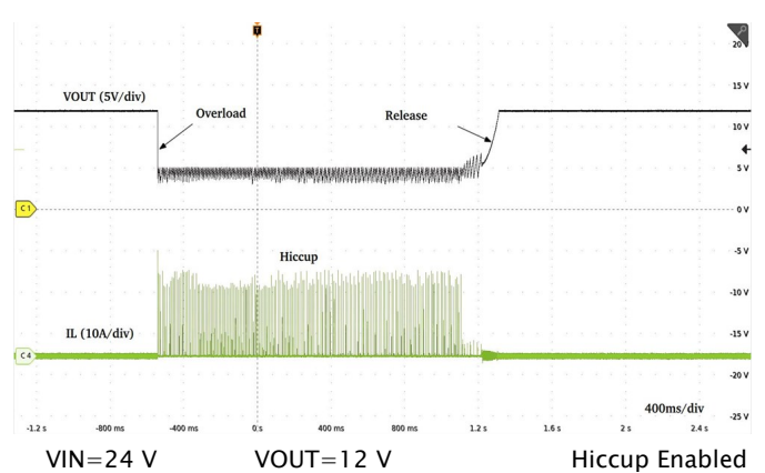
Figure 21. Hiccup Mode Current Limit
