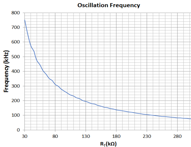
Figure 7. Frequency vs. R_T
