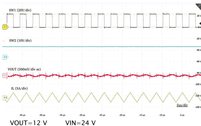
Figure 13. Forced CCM Operation (Buck)
