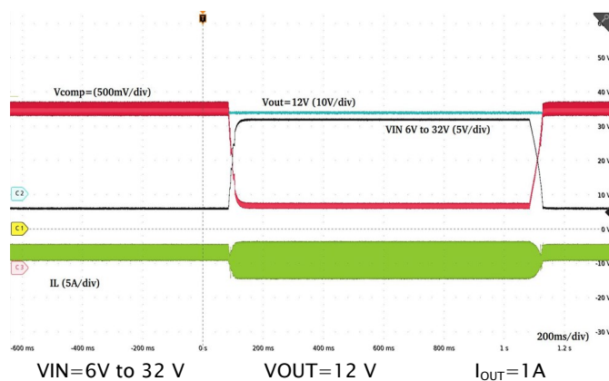
Figure 20. Line Transient
