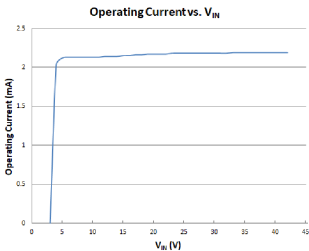
Figure 8. Operating Current vs. V_{IN}
