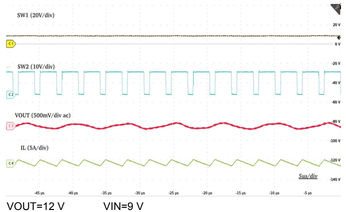
Figure 15. Forced CCM Operation (Boost)
