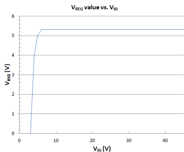
Figure 11. V_{REG} value vs. V_{IN}
