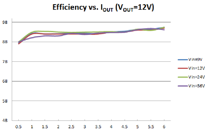
Figure 6. Efficiency
