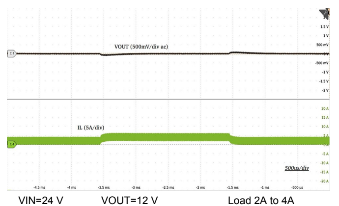
Figure 17. Load Step (Buck)
