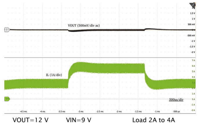
Figure 16. Load Step (Boost)
