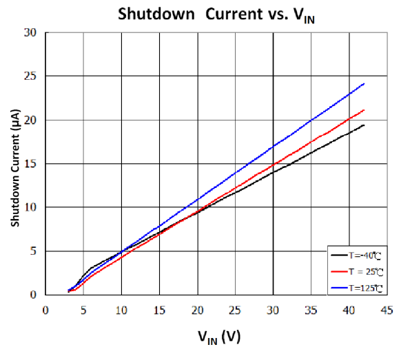
Figure 9. Shutdown Current vs. V_{IN}
