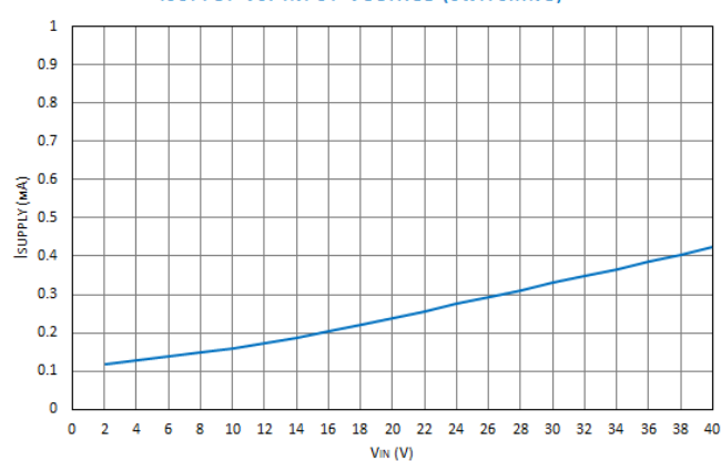
ISUPPLY VS. INPUT VOLTAGE (SWITCHING)
