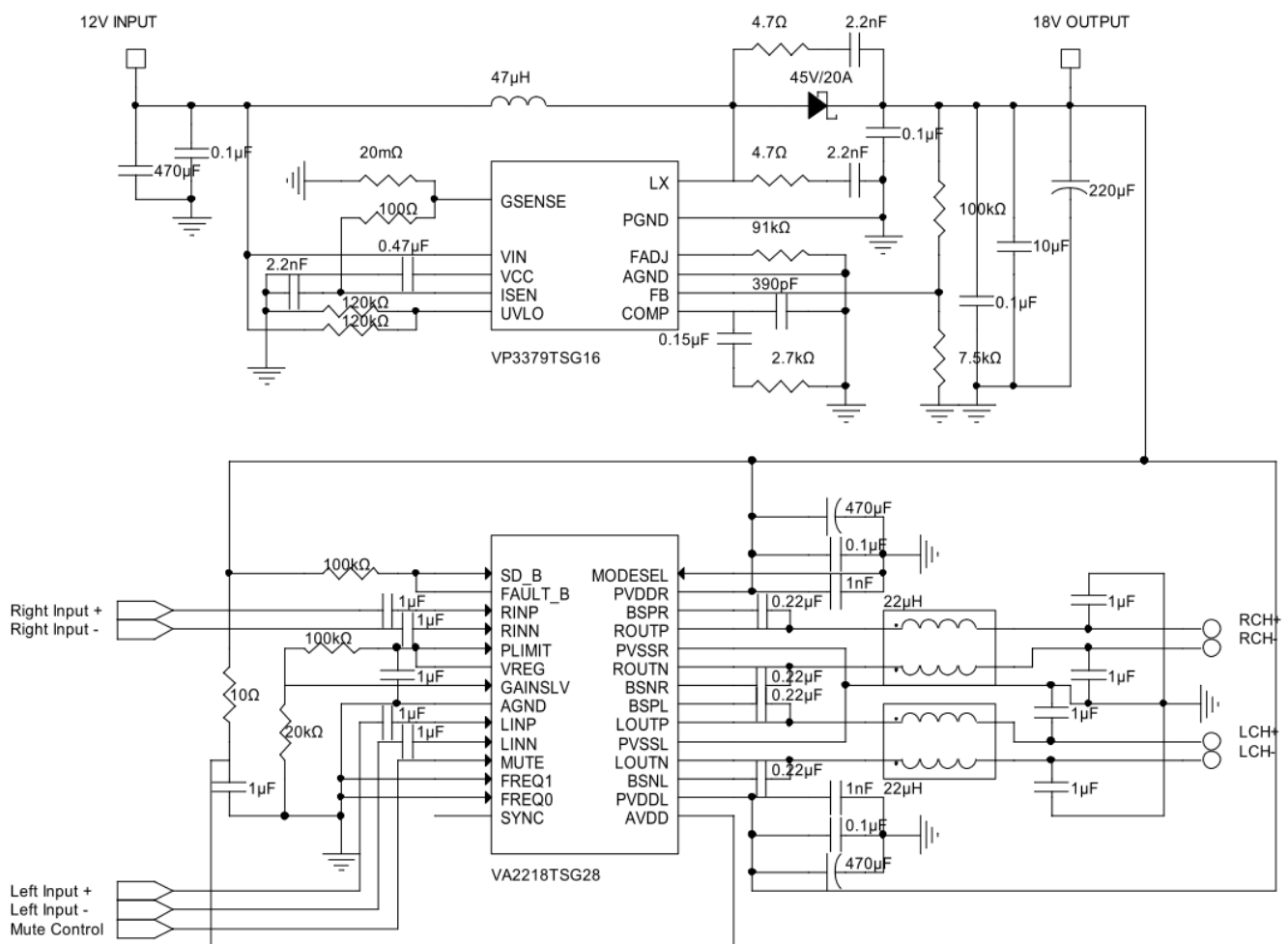
Figure 10. 30W Stereo Class D Amplifier Boosted by VP3379
