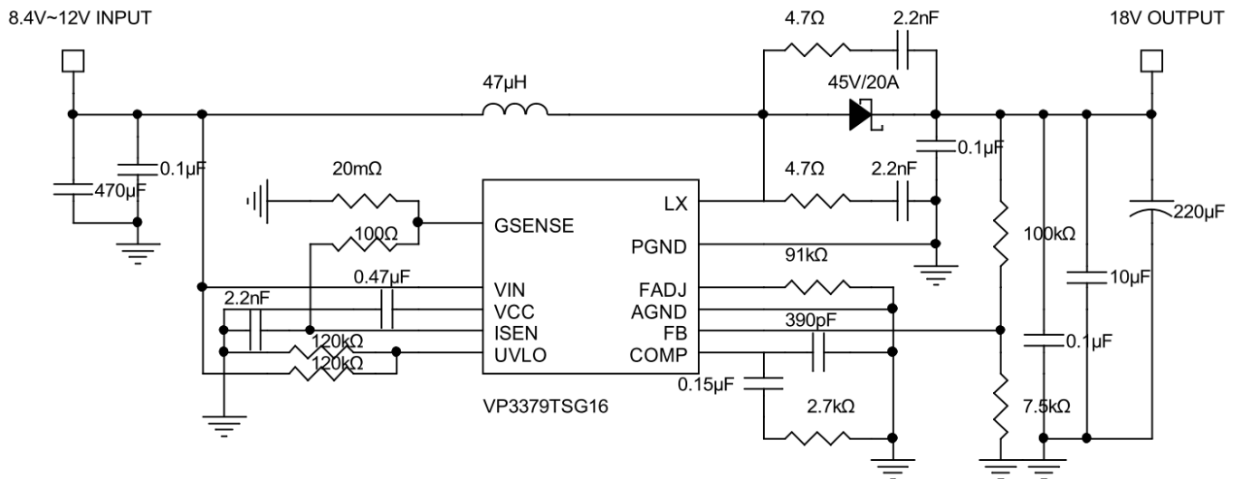
Figure 9. VP3379 18V/3A Boost Reference Application
