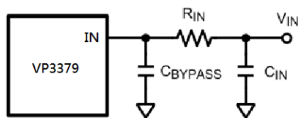
Figure 7 Reducing IC Input Noise
