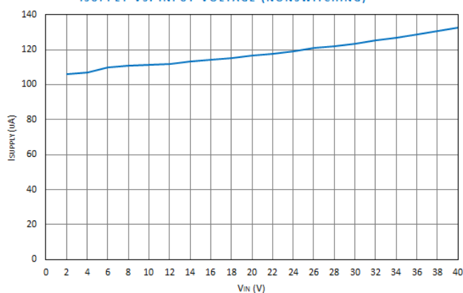
ISUPPLY VS. INPUT VOLTAGE (NONSWITCHING)
