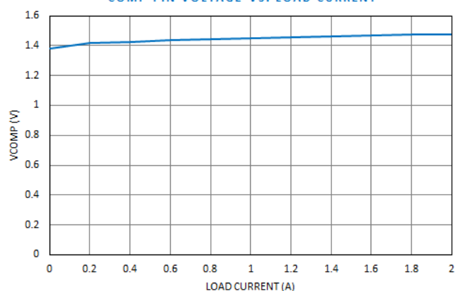
COMP PIN VOLTAGE VS. LOAD CURRENT
