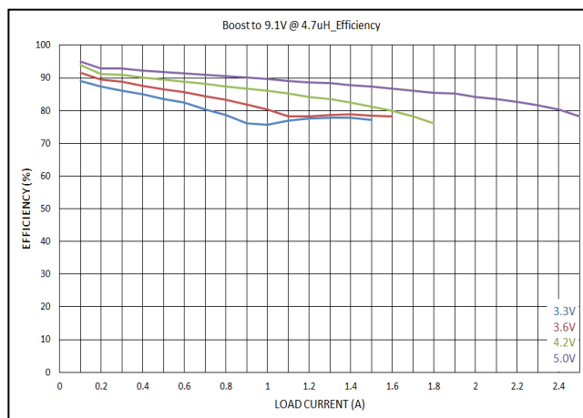
Figure 9. Boost to 9.1V Efficiency vs. Current
