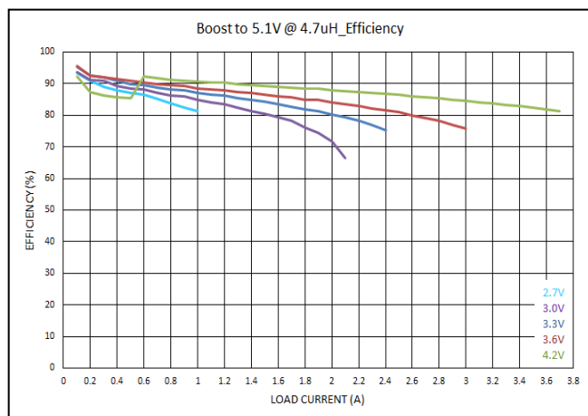
Figure 8. Boost to 5.1V Efficiency vs. Current
