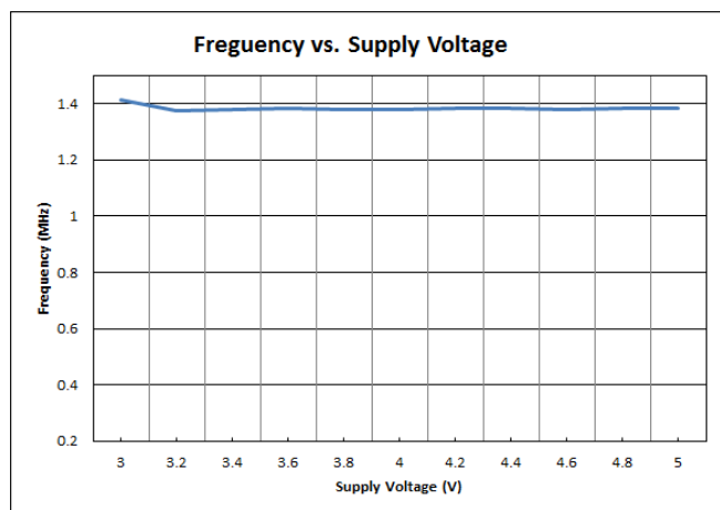
Figure 6. Frequency vs. Supply Voltage
