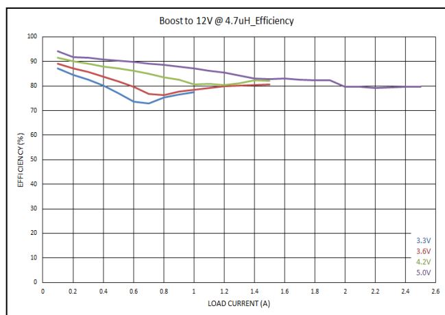
Figure 10. Boost to 12V Efficiency vs. Current
