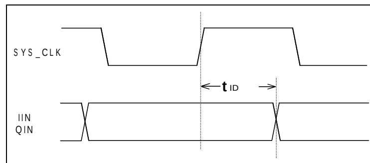
Fig. 22. VP305/6 data input timing diagram.
