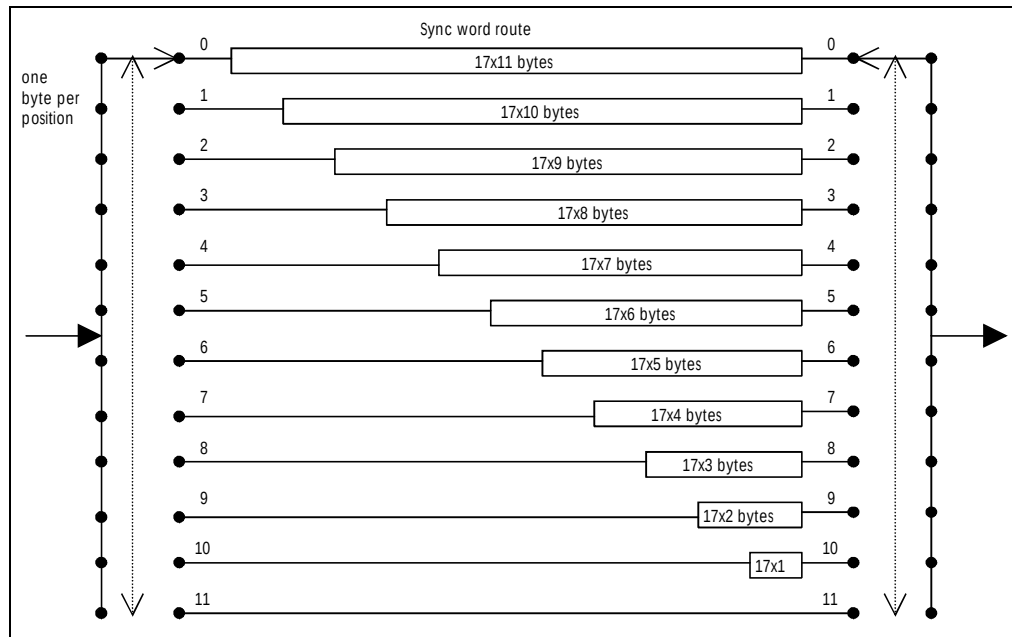
Fig. 10. Conceptual diagram of the convolutional de-interleaver block.
