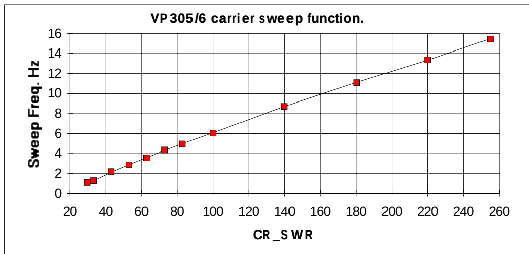
Fig. 16. Carrier sweep rate for a delta frequency of \pm 10\text{MHz} .
