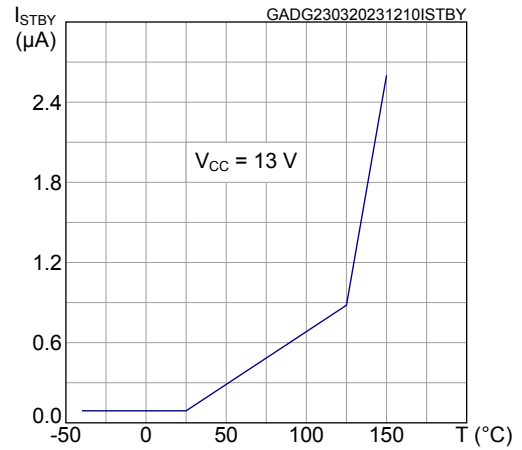
Figure 13. Standby current
