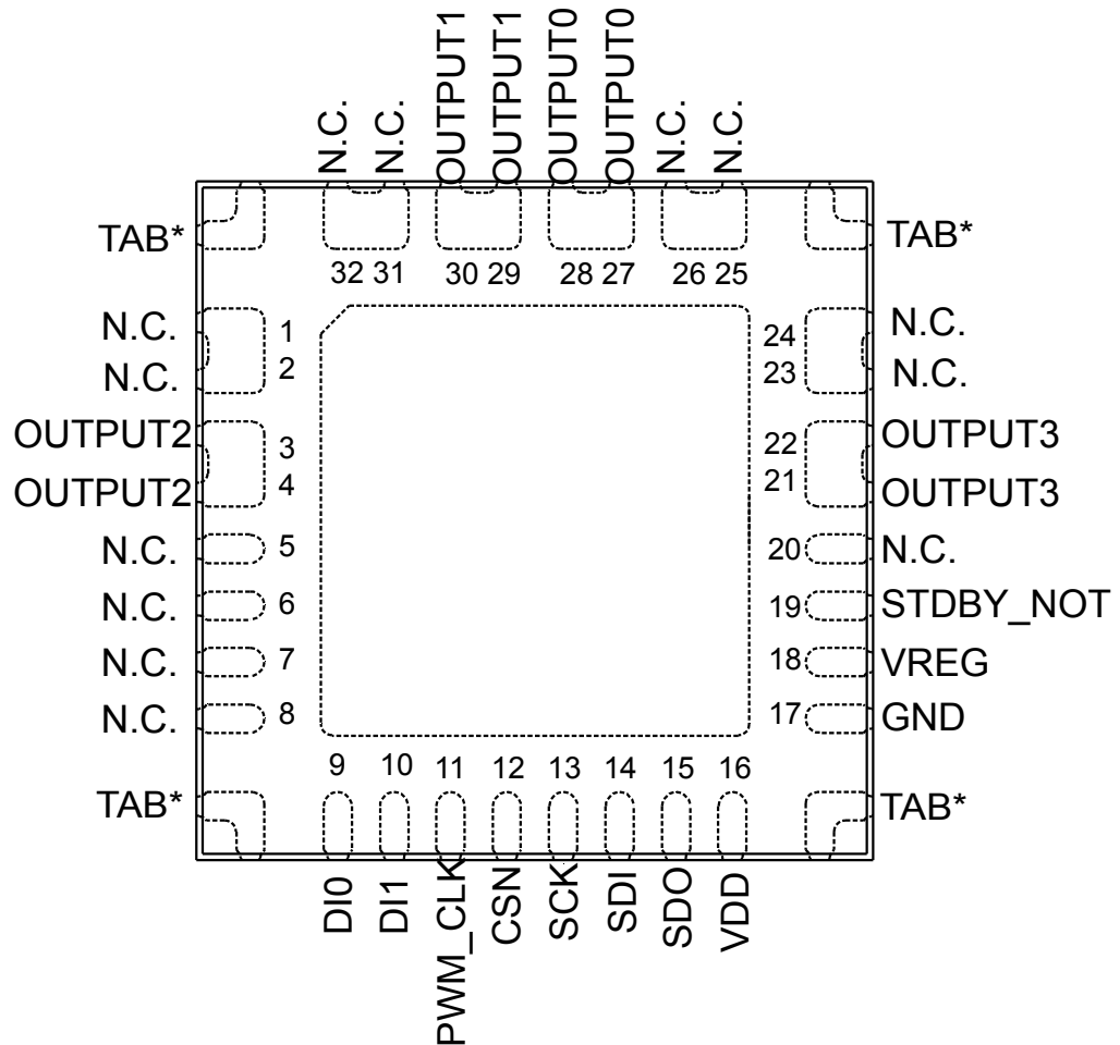
Figure 2. Connection diagram
