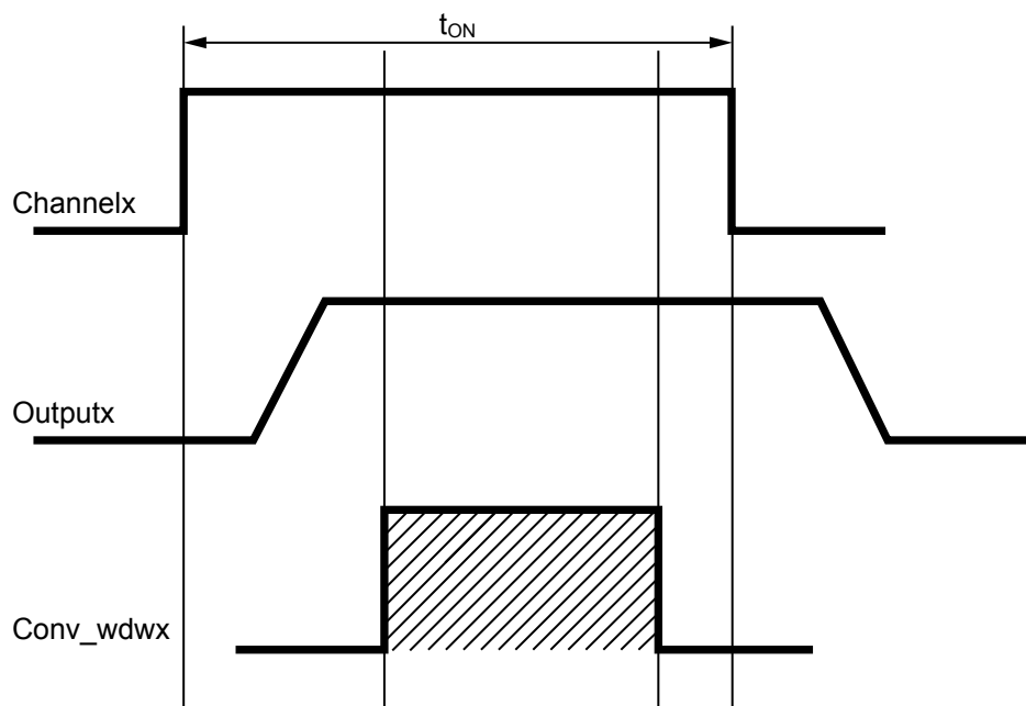
Figure 22. Conversion window generation
