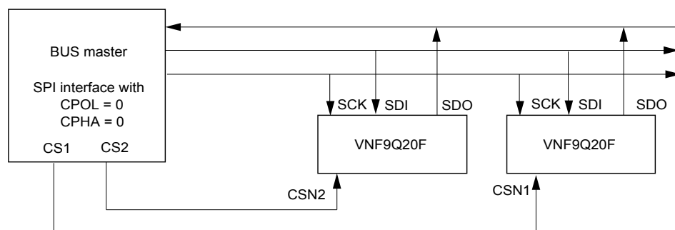
Figure 15. Bus master and two devices in a normal configuration
