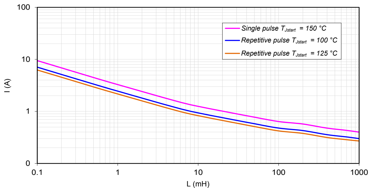
Figure 38. Maximum turn off current versus inductance – Bulb mode
