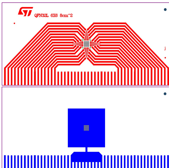
Figure 45. QFN (6x6 mm) PCB 4 layer 2
