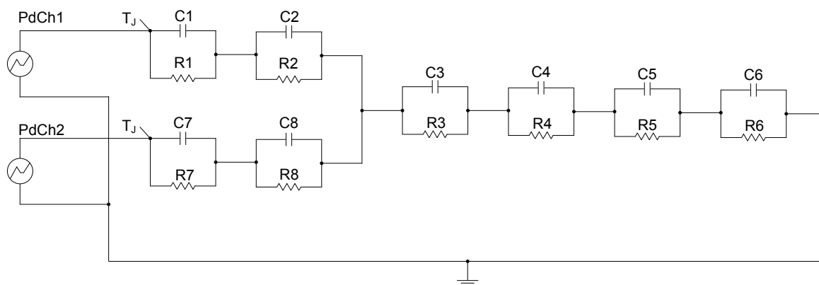
Figure 48. Thermal fitting model
