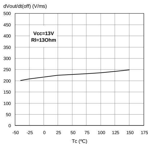
Figure 26. Turn-off Voltage Slope
