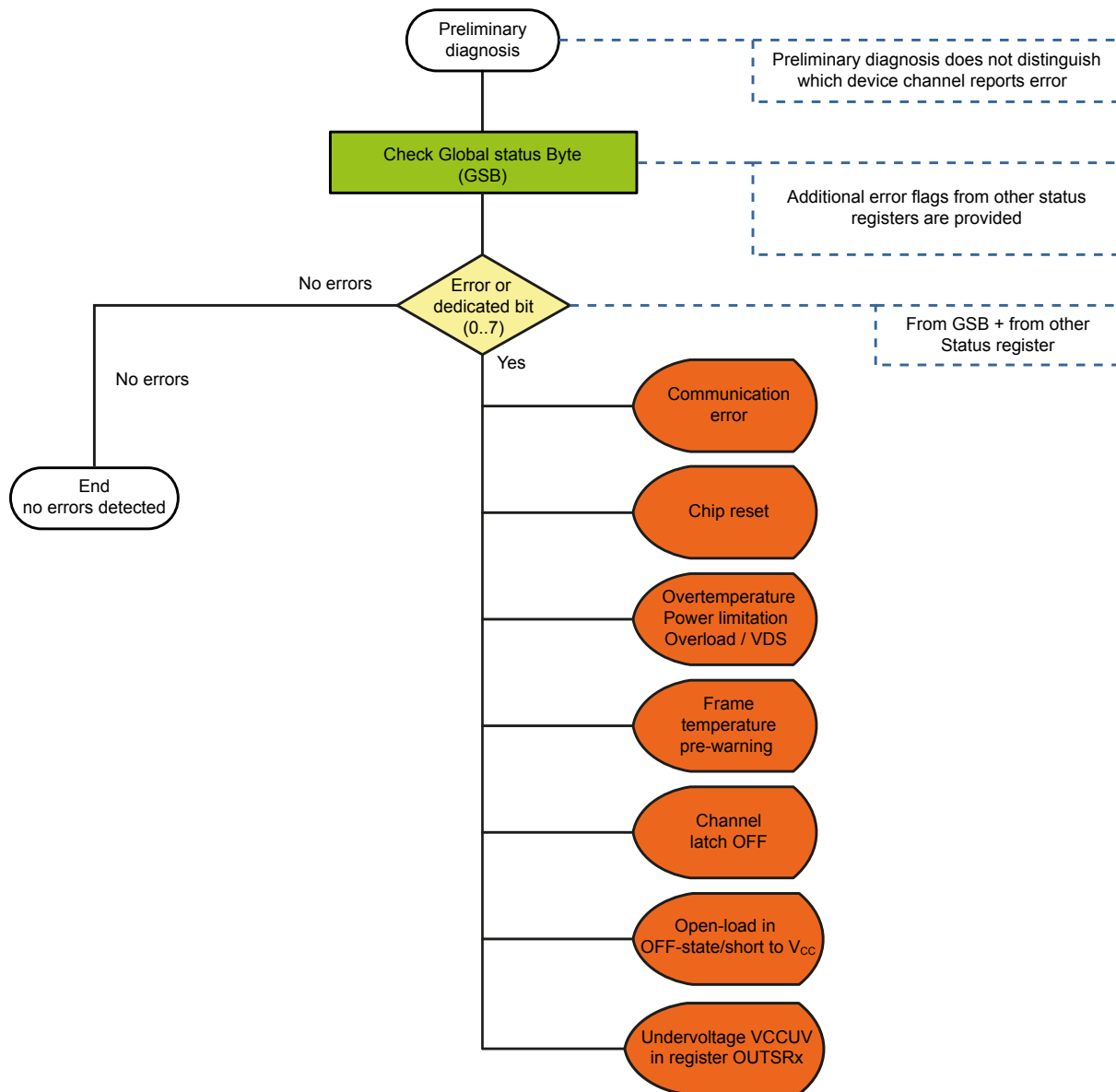
Figure 23. Status registers
