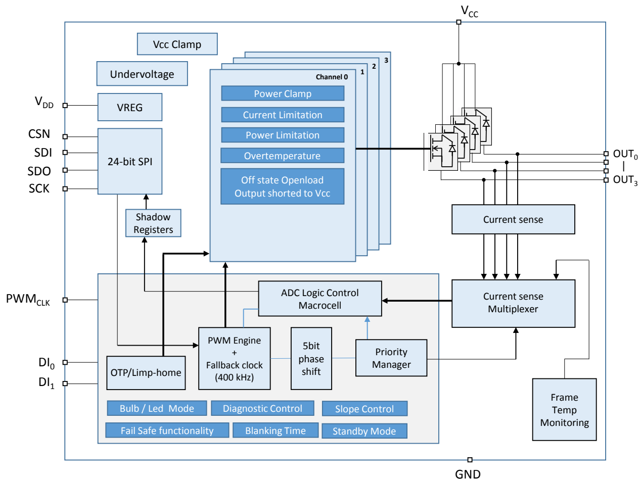
Figure 1. Block diagram
