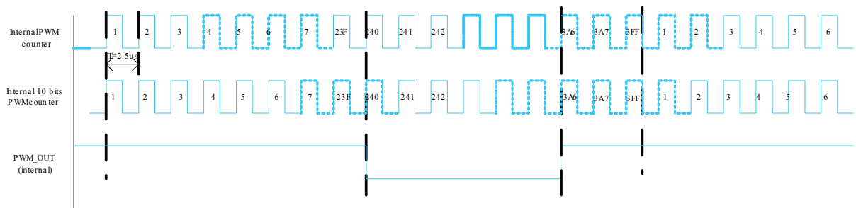
Figure 15. Resulting waveform 4
