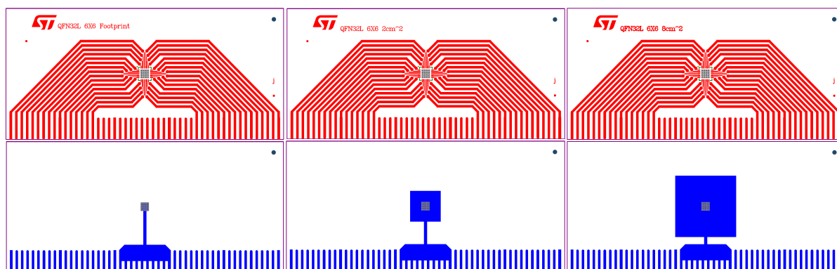
Figure 41. QFN 6x6 PCB 4 layers
