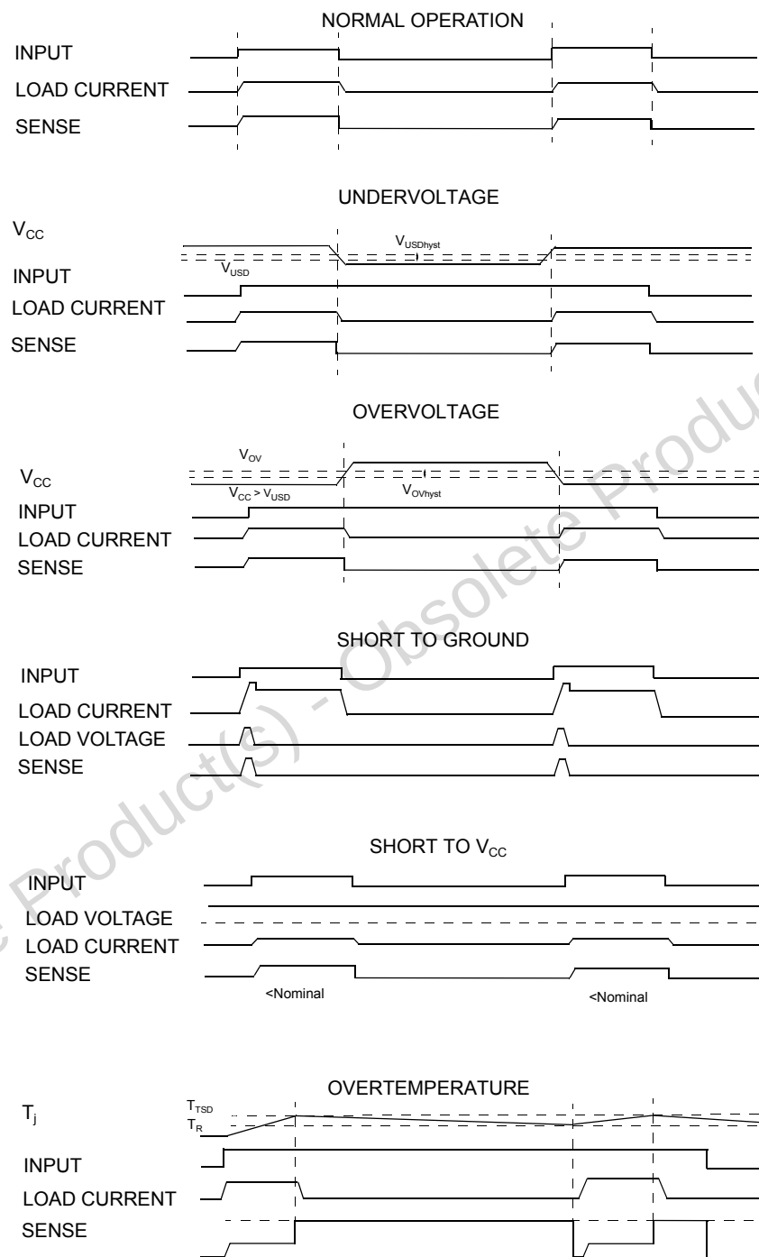
Figure 7. Waveforms
