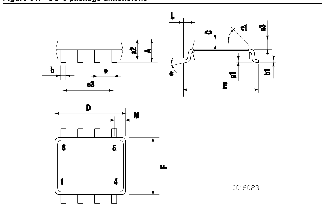
Figure 31. SO-8 package dimensions
