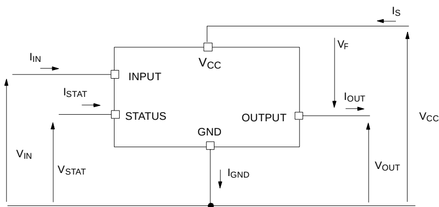
Figure 4. Current and Voltage Conventions
