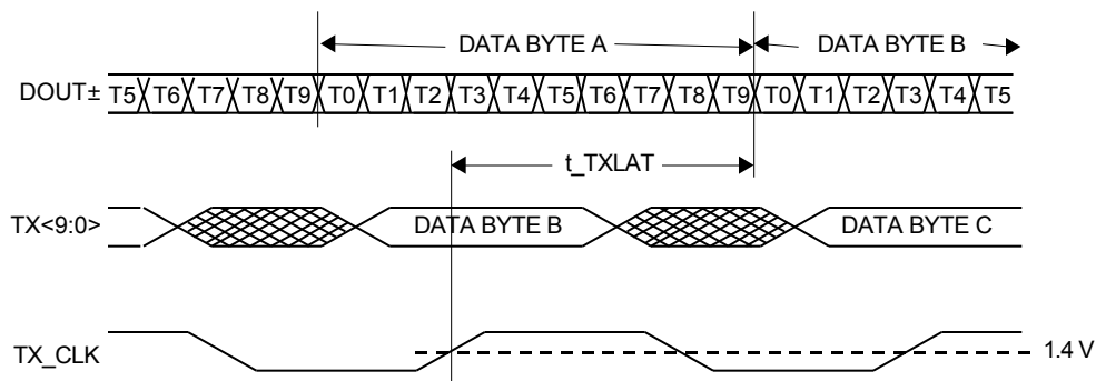
Figure 4. Transmitter Latency
