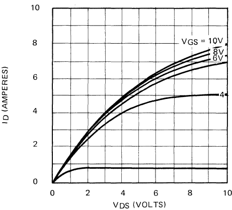
Saturation Characteristics
