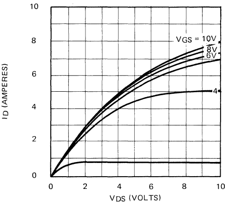
Saturation Characteristics
