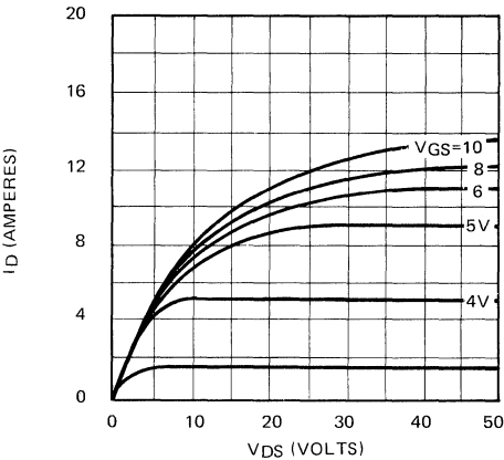
Output Characteristics
