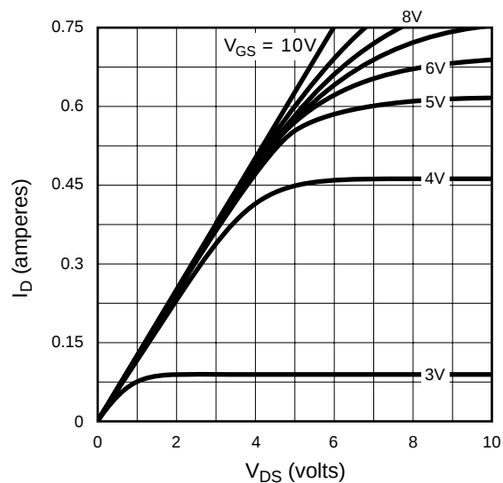
Saturation Characteristics
