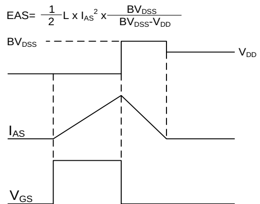
Fig.12 EAS Waveform
