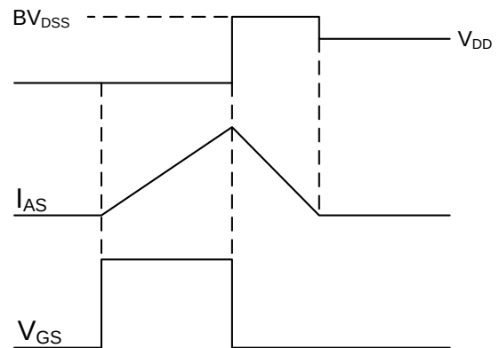
Fig.8 EAS Waveform
