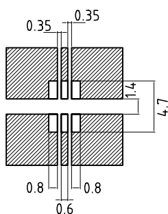
Soldering pads
