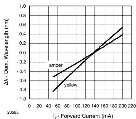
Figure 4. Dominant Wavelength vs. Forward Current
