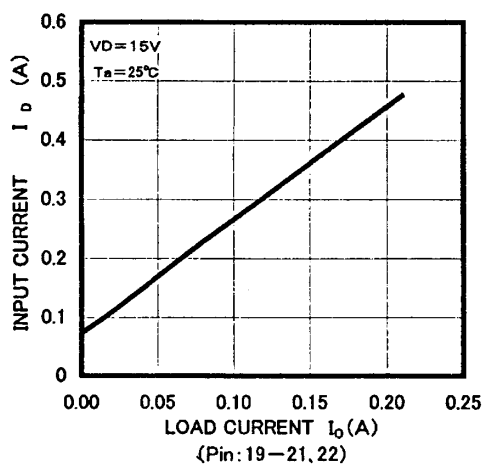
I_D - I_D CHARACTERISTICS (TYPICAL)
