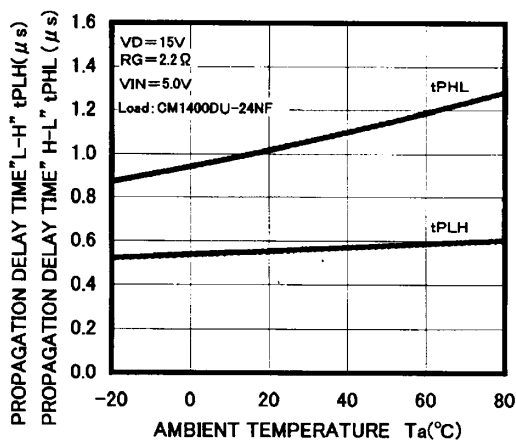
t_{PLH}, t_{PHL} - T_a CHARACTERISTICS (TYPICAL)
