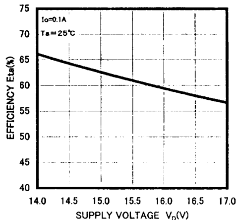
\eta_a - V_D CHARACTERISTICS (TYPICAL)
