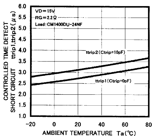
t_{trip} - T_a CHARACTERISTICS (TYPICAL)
