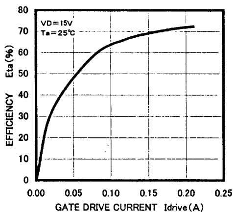
\eta_a - I_{drive} CHARACTERISTICS (TYPICAL)
