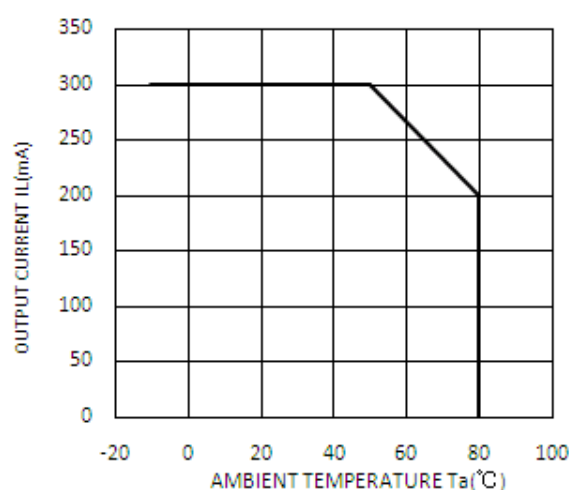
DERATING CHARACTERISTICS
