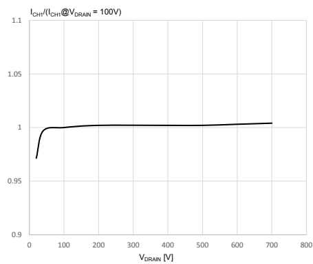
Figure 11. I_{CH1} vs. V_{DRAIN}
