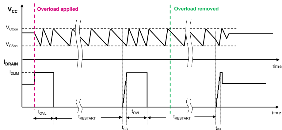
Figure 30. Overload protection
