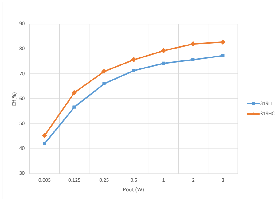
Figure 28. Light load efficiency @ 230VAC
