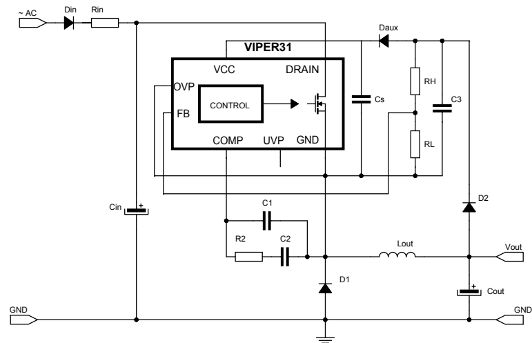
Figure 42. Buck converter
