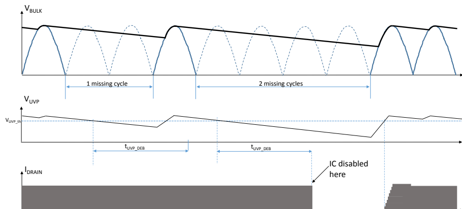
Figure 33. Hold-up in case of input line missing cycles
