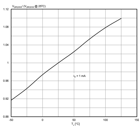
Figure 19. V_{BVDSS} vs. T_J
