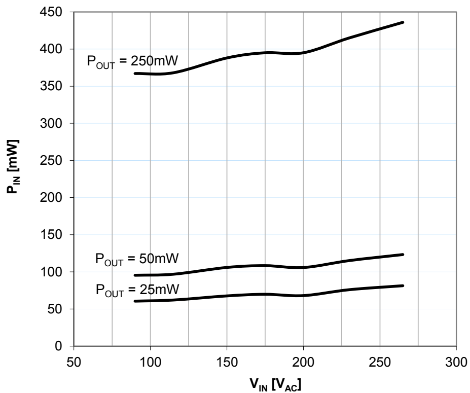
Figure 45. Input power vs V_{IN} in light-load conditions, V_{OUT} = 15V
