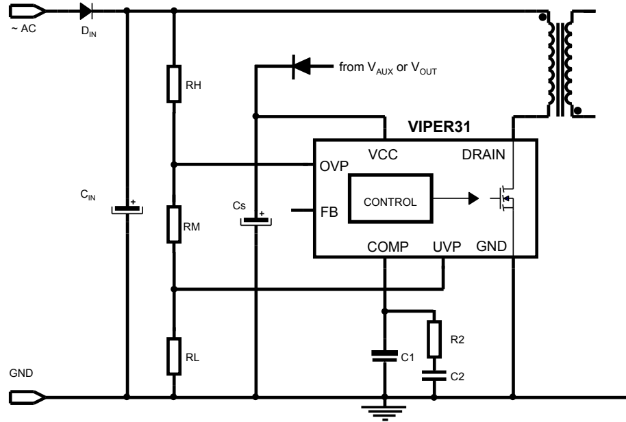
Figure 37. Connection for input and output overvoltage protections (iso/non-iso topologies)
