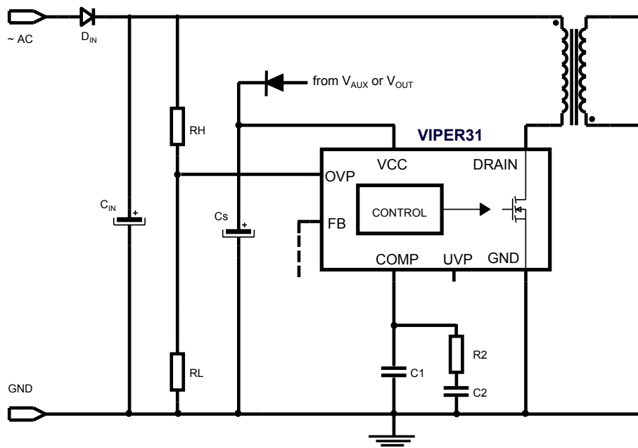
Figure 35. Connection for input overvoltage protection (iso/non-iso topologies)
