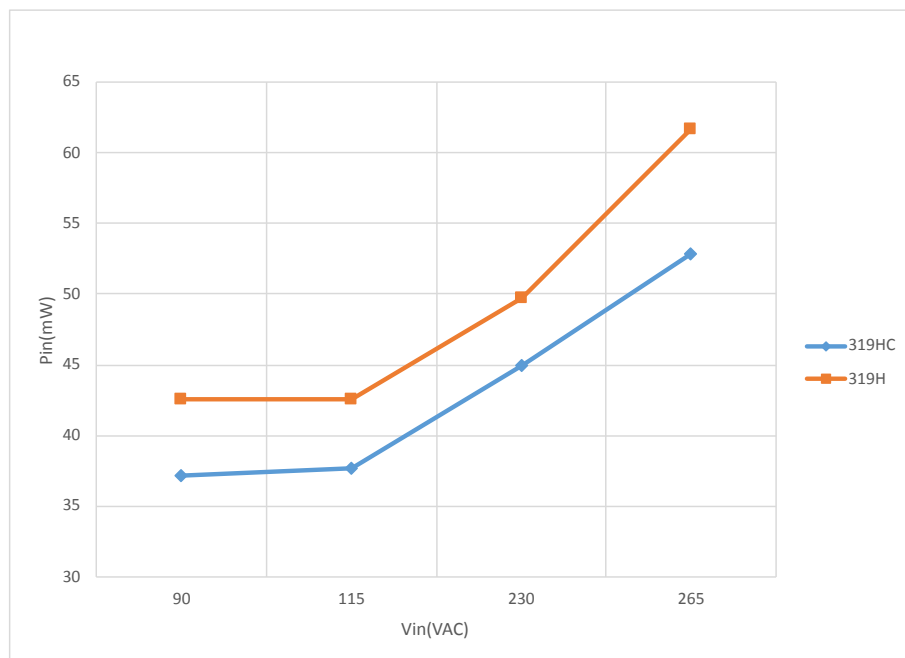
Figure 29. No load input power vs input voltage
