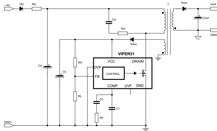
Figure 41. Flyback converter (primary regulation)
