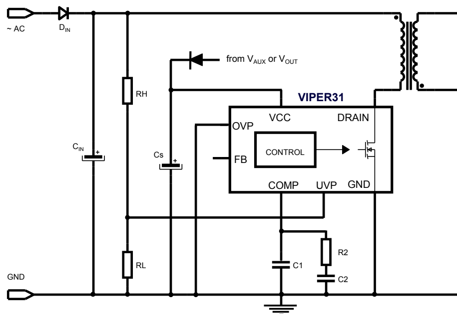
Figure 32. Connection for input undervoltage protection/disable (isolated or non-isolated topologies)
