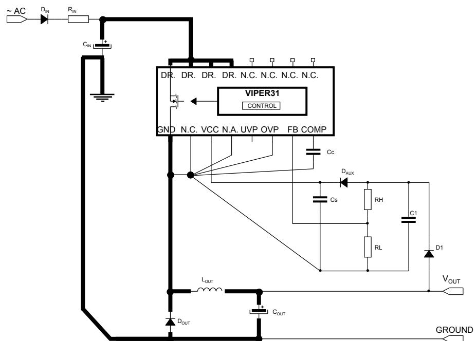
Figure 47. Recommended routing for buck converter
