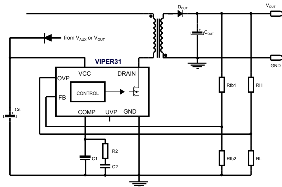
Figure 36. Connection for output overvoltage protection (non-iso topologies)
