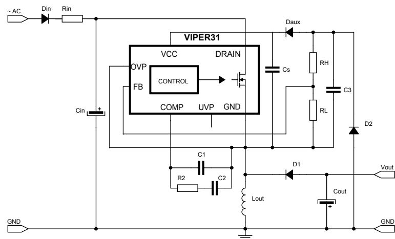
Figure 43. Buck-boost converter
