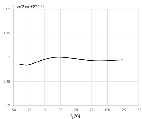
Figure 4. F_{OSC} vs. T_J
