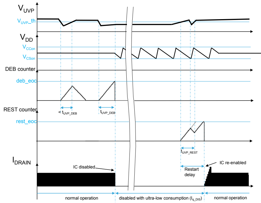
Figure 31. UVP timing
