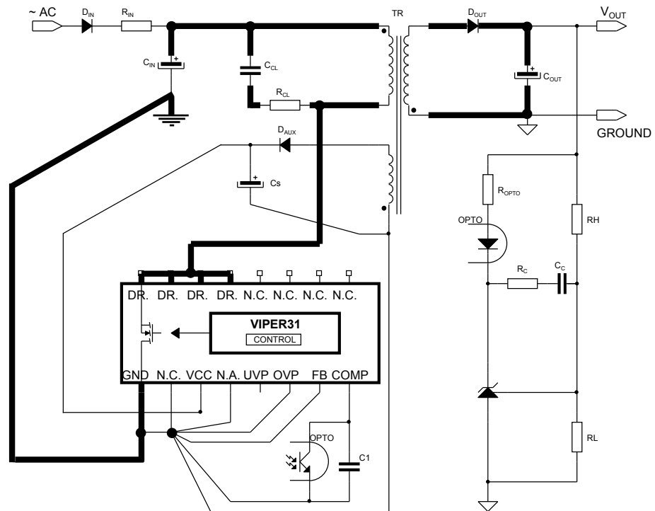
Figure 46. Recommended routing for flyback converter
