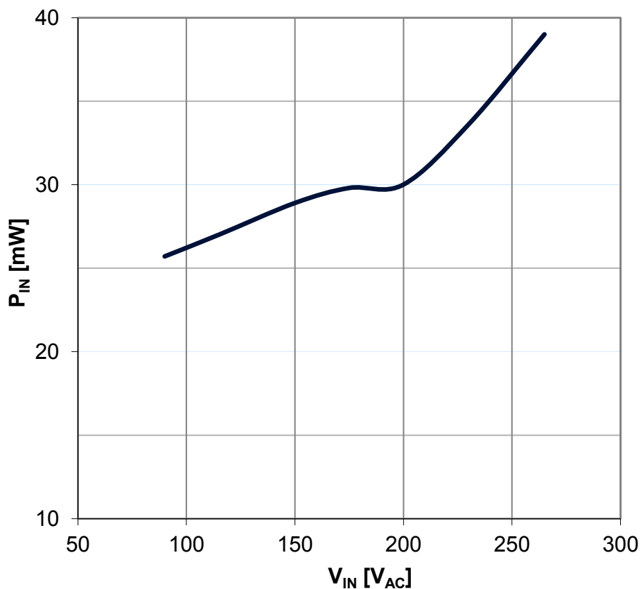
Figure 44. Input power vs V_{IN} in no-load condition, V_{OUT} = 15\text{ V}
