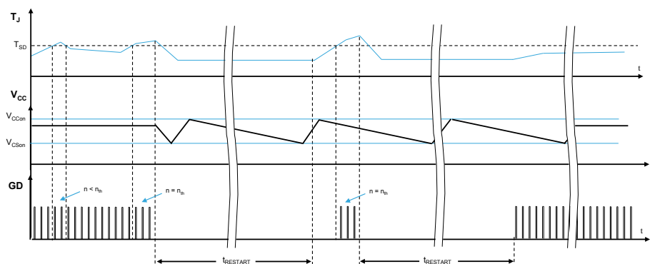
Figure 38. Thermal shutdown timing diagram
