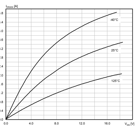
Figure 20. Output characteristic
