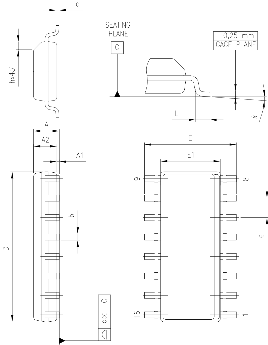
Figure 48. SO16N package outline
