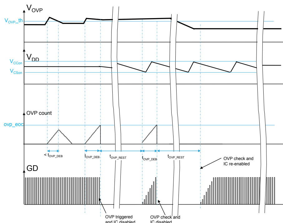
Figure 34. OVP timing
