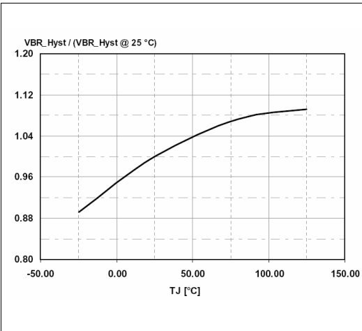
Figure 11. Brown-out hysteresis vs T_J
