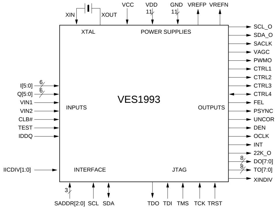
FIGURE 2. BLOCK DIAGRAM
