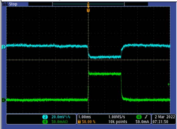
Fig 9. Load Transient
