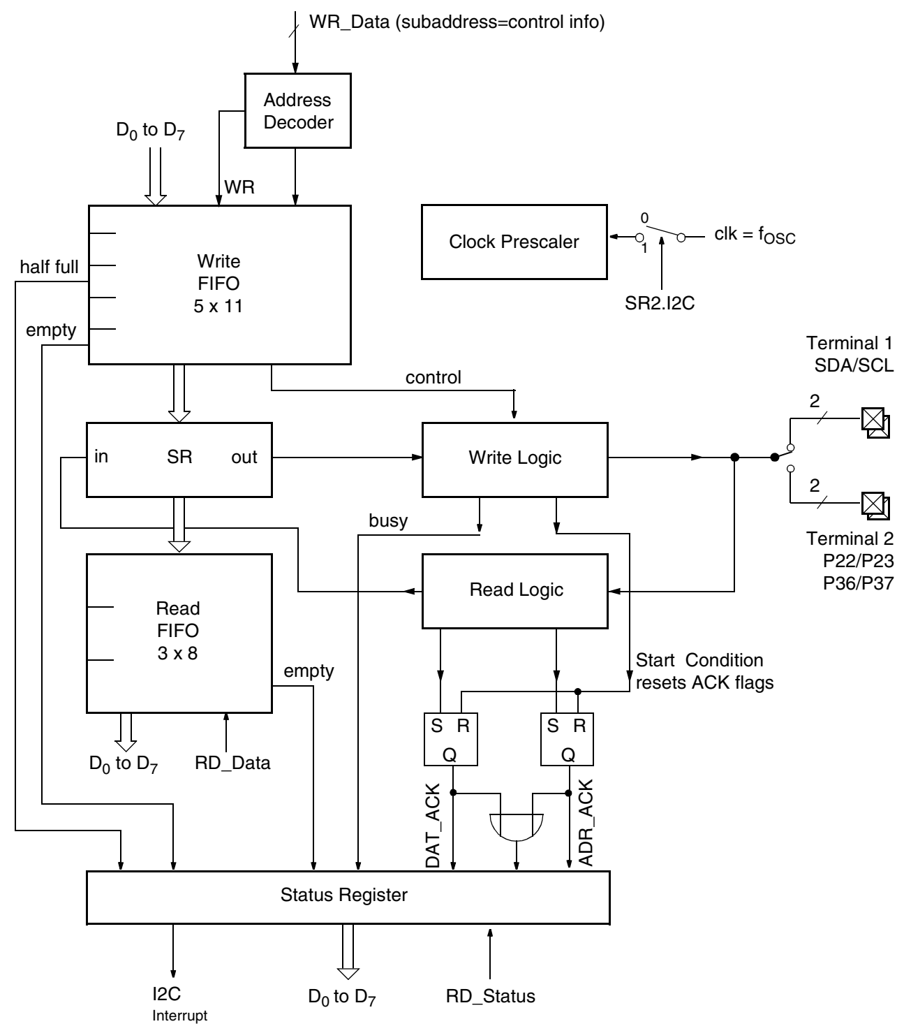
Fig. 5–18: Block diagram of I²C bus master interface
