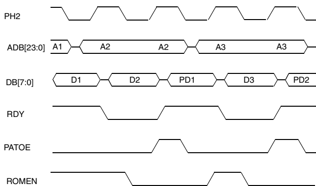
Fig. 5–17: Patch timing
