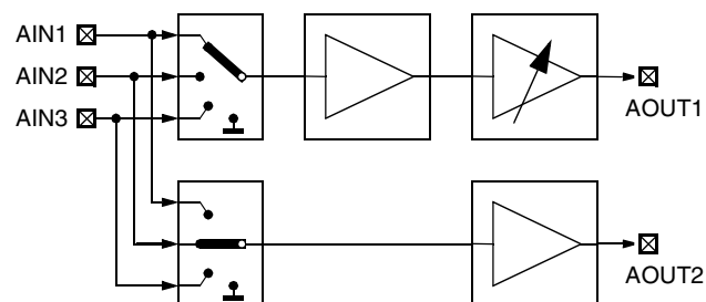
Fig. 4–1: Audio processing
