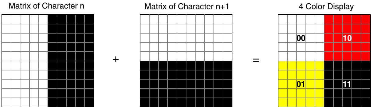
Fig. 3–20: Four-color mode
