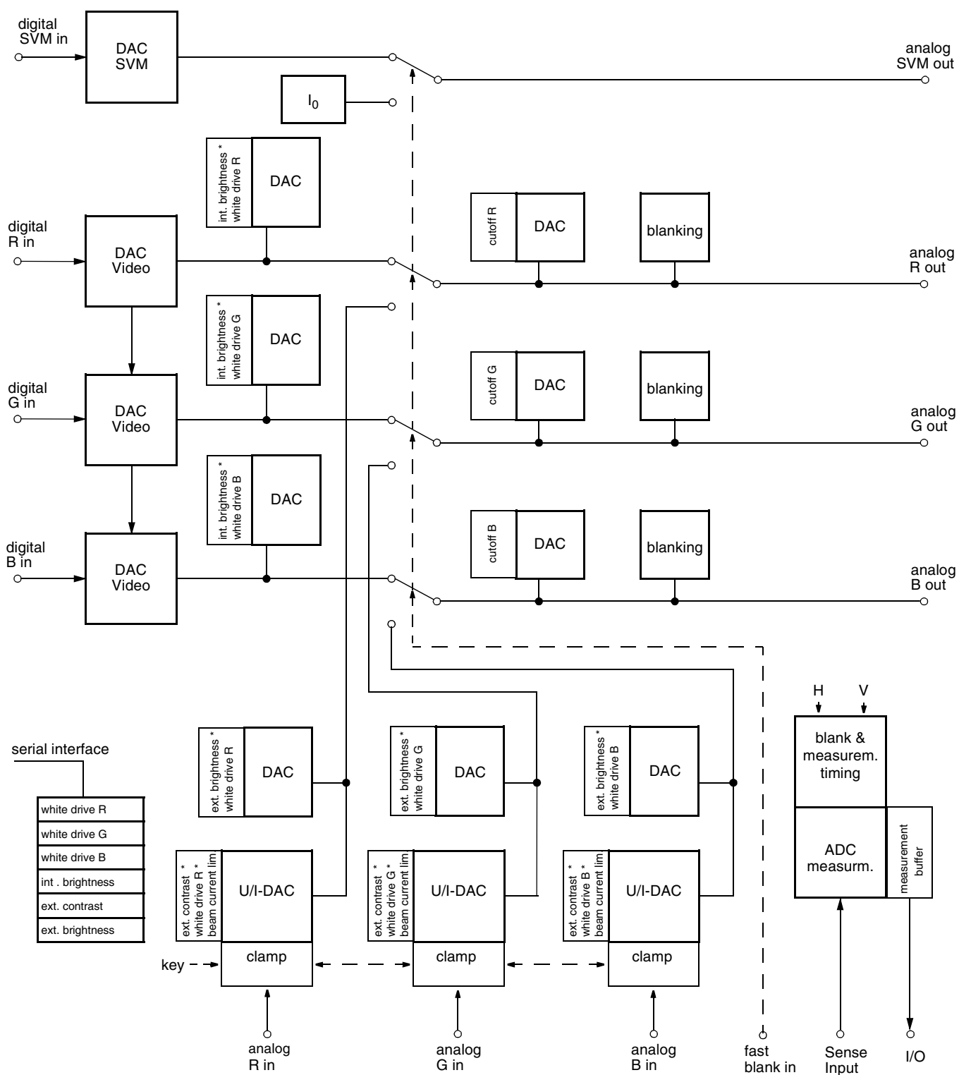
Fig. 2-23: Video back-end
