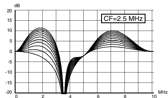
Fig. 2-14: Total frequency response for peaking filter and S-VHS, PAL, NTSC
