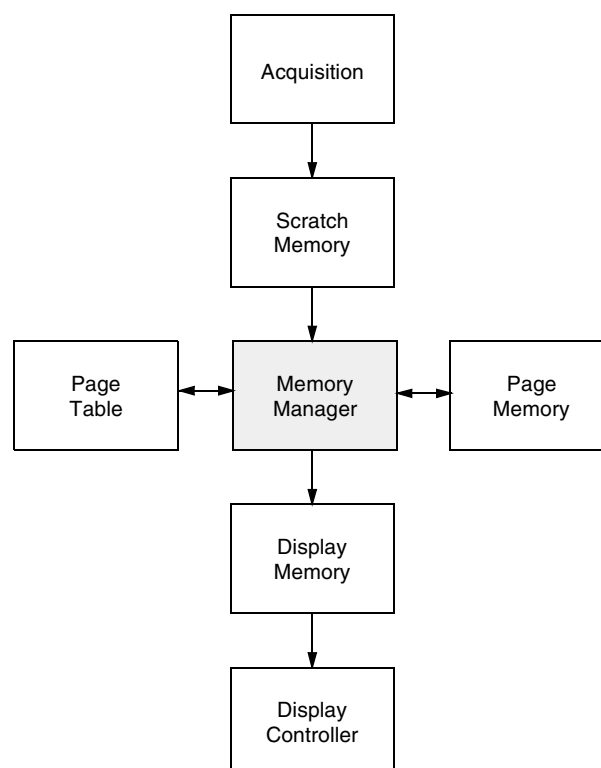
Fig. 3-3: Memory Manager
