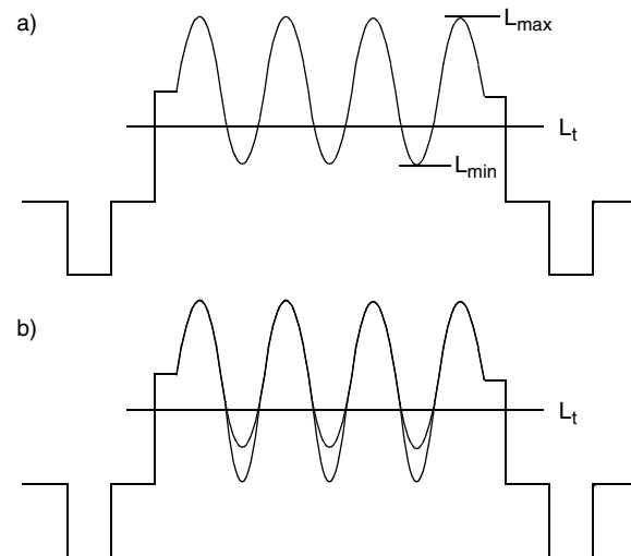
Fig. 2-12: Black-level expansion
