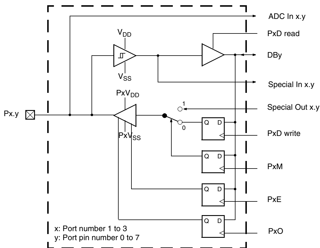
Fig. 5–29: Universal port circuit
