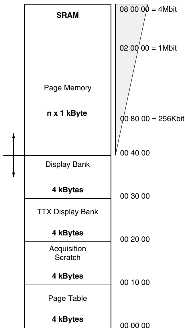
Fig. 3–4: Memory organization
