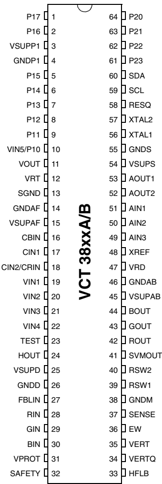
Fig. 6-3: PSDIP64 package
