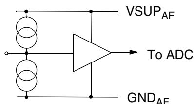
Fig. 6-11: Input pins CRIN, CBIN
