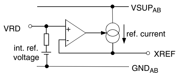
Fig. 6-24: Supply pins XREF, VRD
