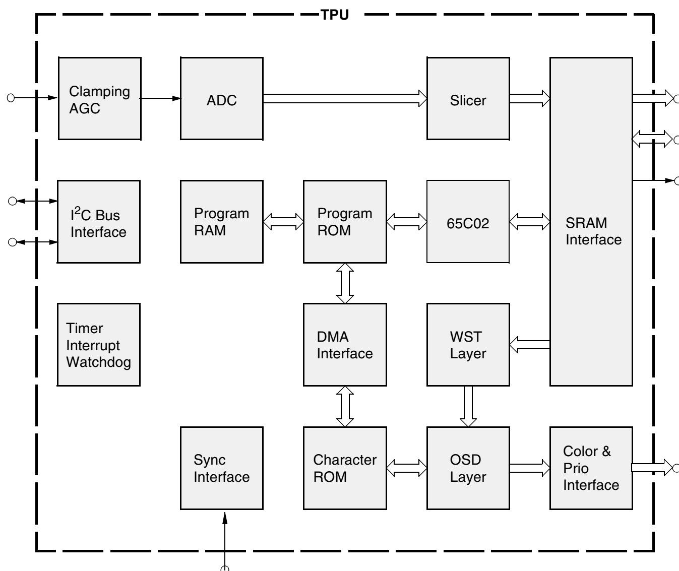
Fig. 3–1: Block diagram of the TPU
