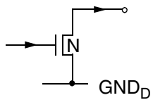
Fig. 6-16: Output pin HOUT
