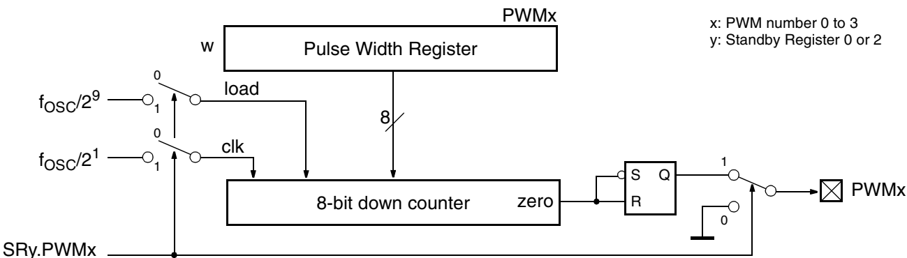
Fig. 5–24: Block diagram of 8-bit PWM
