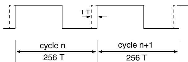
Fig. 5–25: TVPWM Timing
