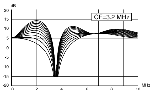
Fig. 2-14: Total frequency response for peaking filter and S-VHS, PAL, NTSC
