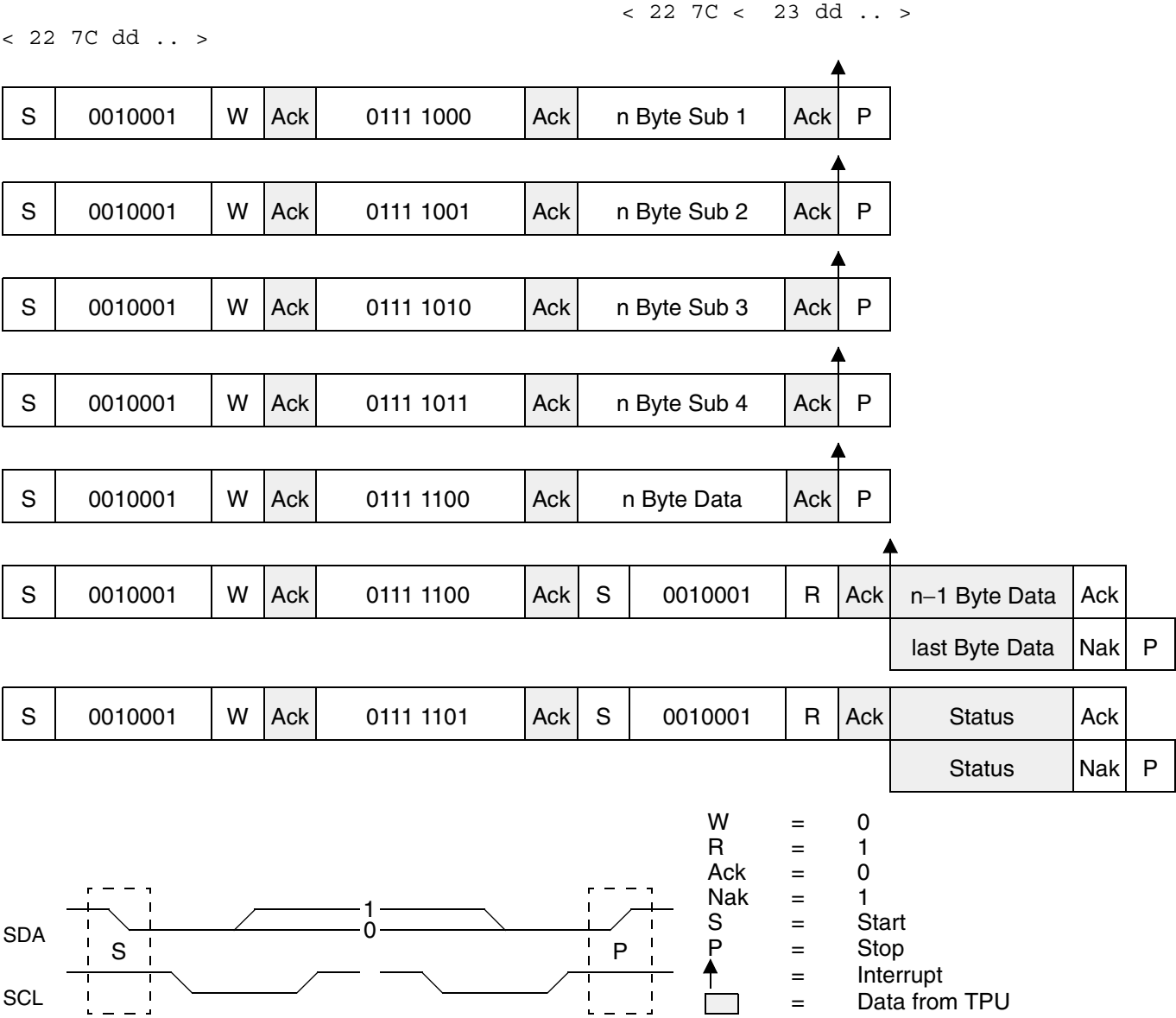
Fig. 3–23: I 2 C bus protocol
