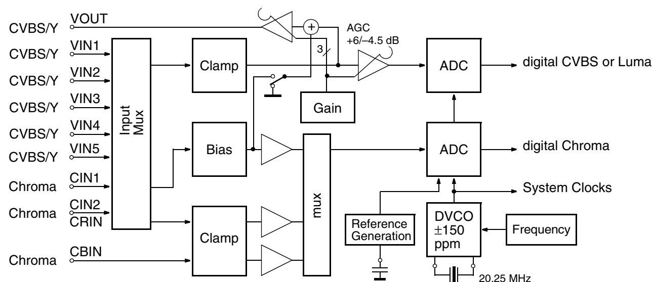
Fig. 2–1: Video front-end
