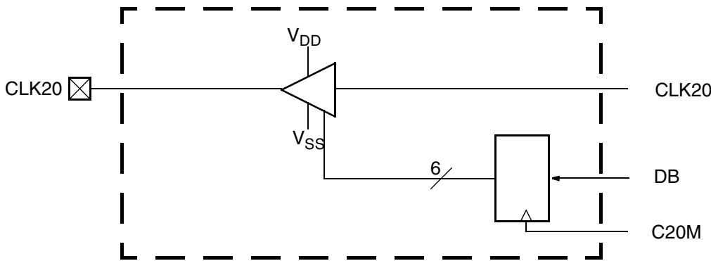
Fig. 5-32: CLK20 Port Circuit
