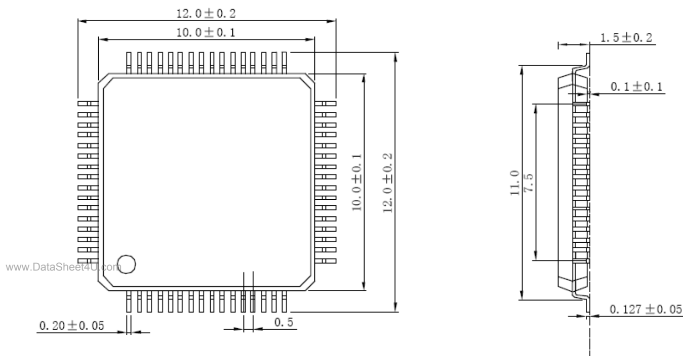
Figure 6-1 LQFP64 Package Information
